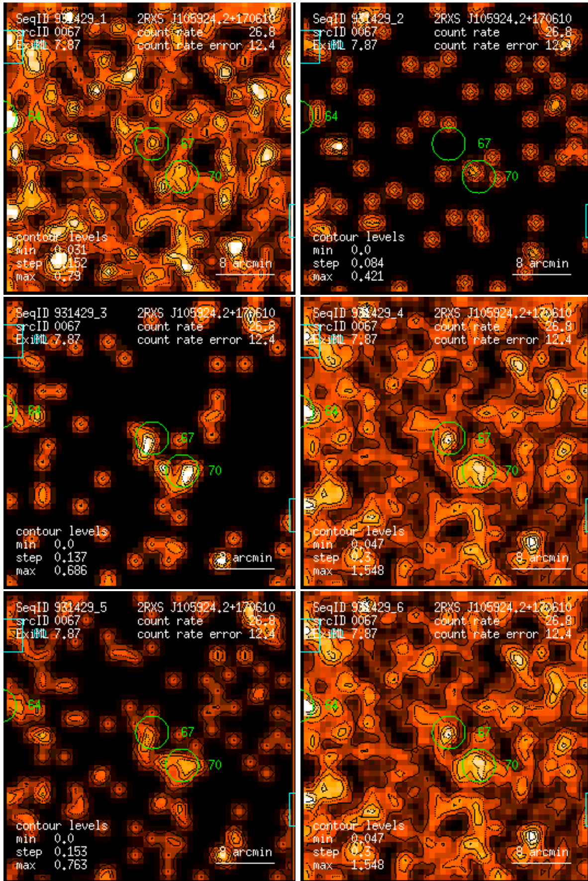
Figure 67: RASS 931429: detection 0067: band rate images, Gaussian filter: (1) PSPC channels 11 – 41, (2) 52 – 90, (3) 91 – 201, (4) 11 – 235, (5) 52 – 201, (6) 11 – 201. Broad band rates in counts/ks. Band rate contour levels in counts/ks/arcmin 2 .
