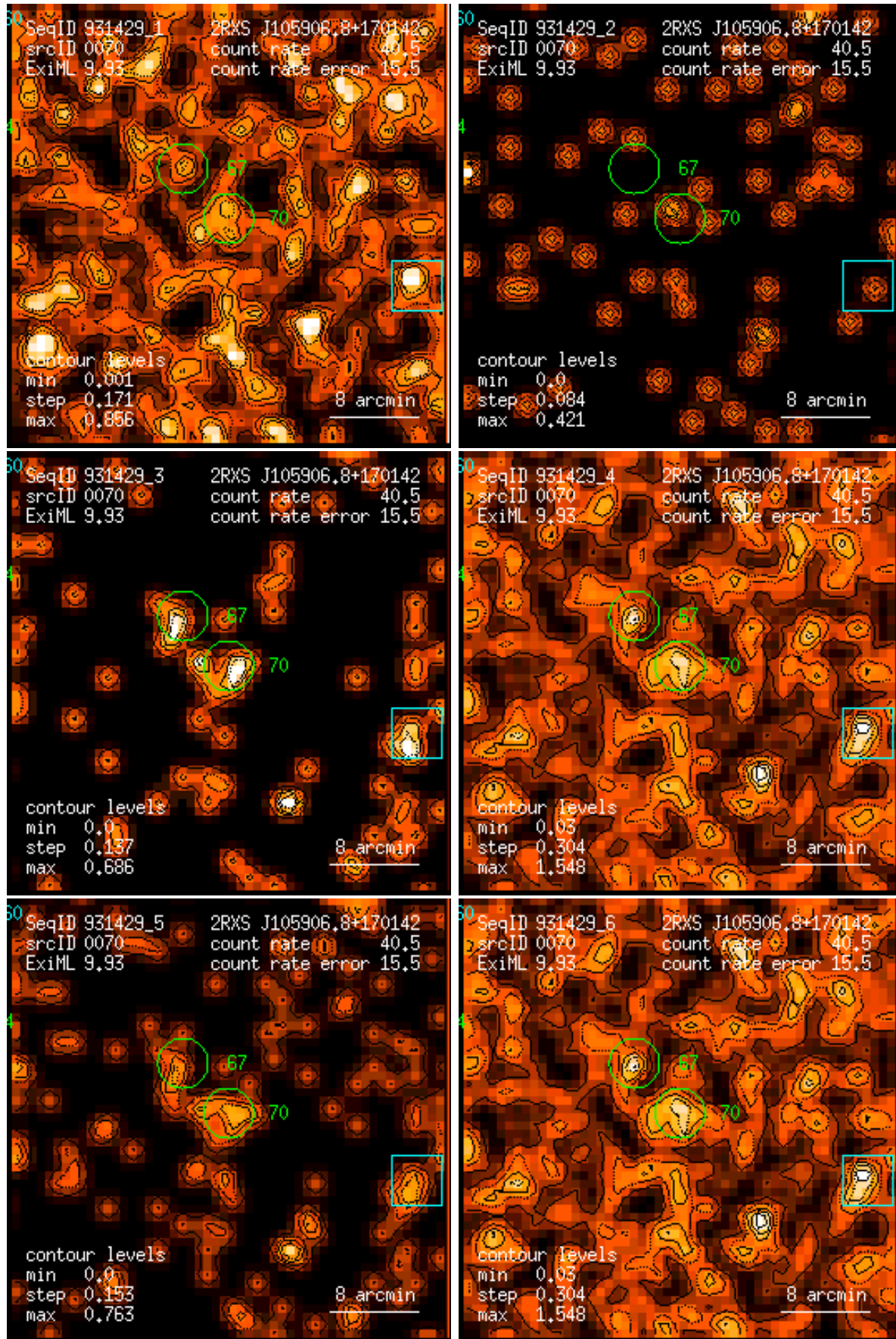
Figure 70: RASS 931429: detection 0070: band rate images, Gaussian filter: (1) PSPC channels 11 – 41, (2) 52 – 90, (3) 91 – 201, (4) 11 – 235, (5) 52 – 201, (6) 11 – 201. Broad band rates in counts/ks. Band rate contour levels in counts/ks/arcmin 2 .
