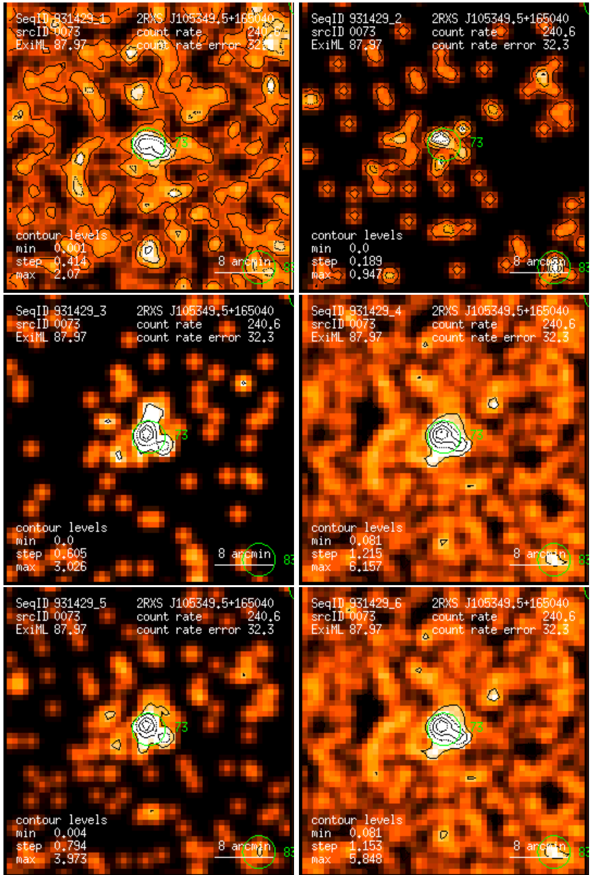
Figure 73: RASS 931429: detection 0073: band rate images, Gaussian filter: (1) PSPC channels 11 – 41, (2) 52 – 90, (3) 91 – 201, (4) 11 – 235, (5) 52 – 201, (6) 11 – 201. Broad band rates in counts/ks. Band rate contour levels in counts/ks/arcmin 2 .
