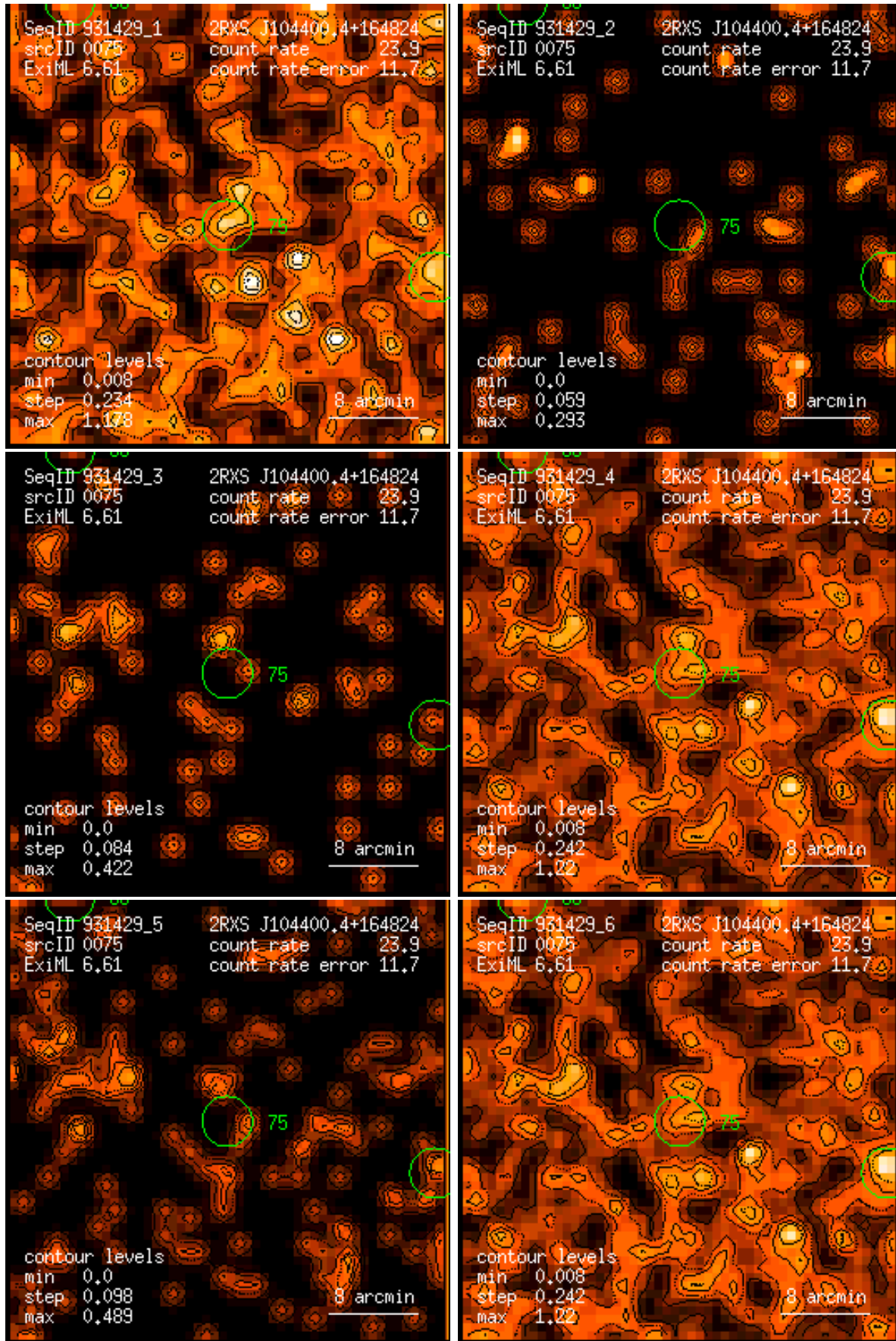
Figure 75: RASS 931429: detection 0075: band rate images, Gaussian filter: (1) PSPC channels 11 – 41, (2) 52 – 90, (3) 91 – 201, (4) 11 – 235, (5) 52 – 201, (6) 11 – 201. Broad band rates in counts/ks. Band rate contour levels in counts/ks/arcmin 2 .
