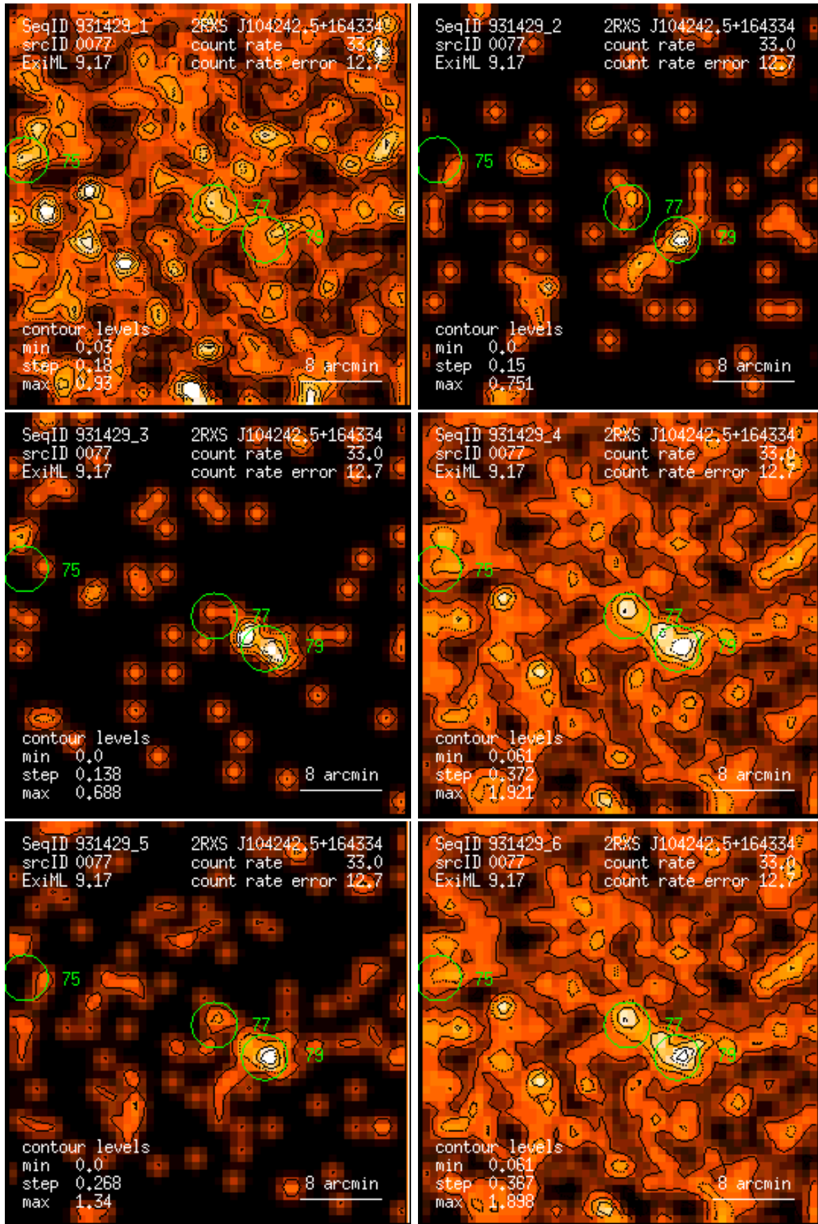
Figure 77: RASS 931429: detection 0077: band rate images, Gaussian filter: (1) PSPC channels 11 – 41, (2) 52 – 90, (3) 91 – 201, (4) 11 – 235, (5) 52 – 201, (6) 11 – 201. Broad band rates in counts/ks. Band rate contour levels in counts/ks/arcmin 2 .
