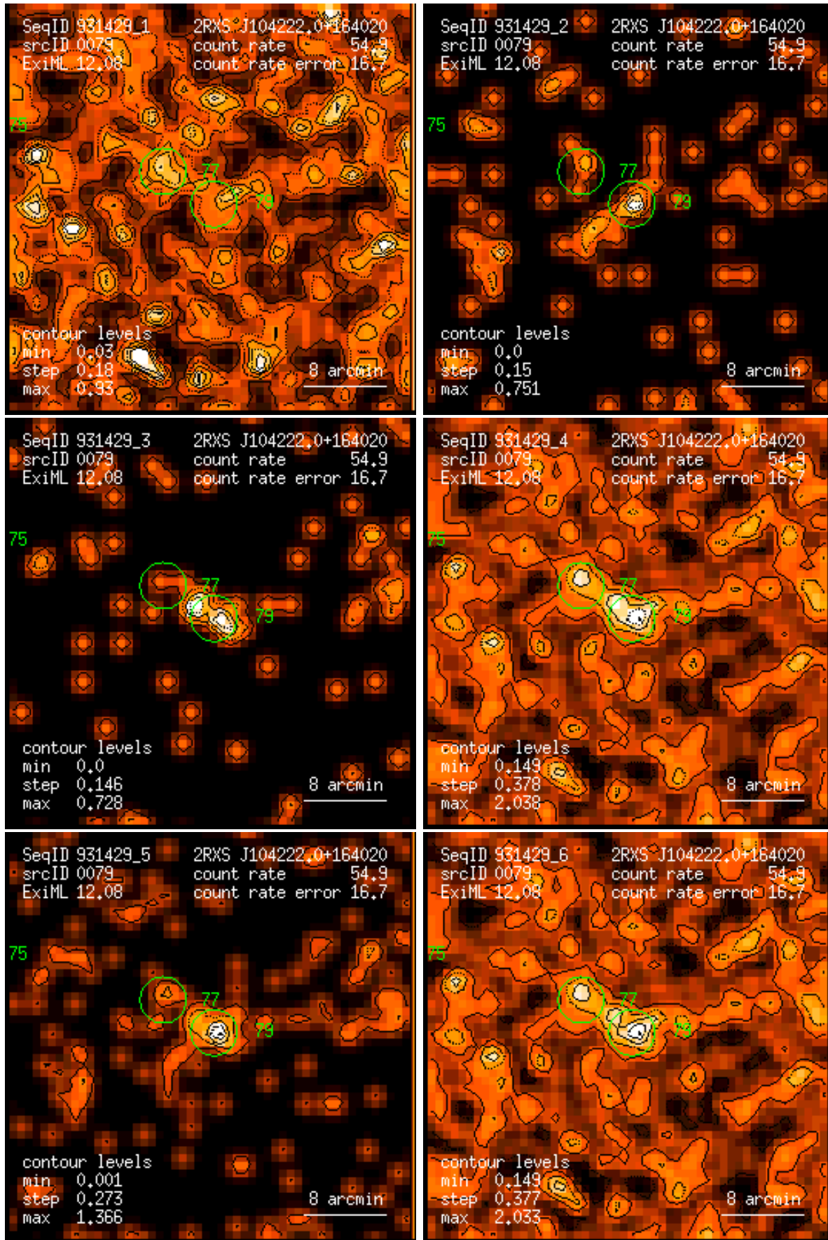
Figure 79: RASS 931429: detection 0079: band rate images, Gaussian filter: (1) PSPC channels 11 – 41, (2) 52 – 90, (3) 91 – 201, (4) 11 – 235, (5) 52 – 201, (6) 11 – 201. Broad band rates in counts/ks. Band rate contour levels in counts/ks/arcmin 2 .
