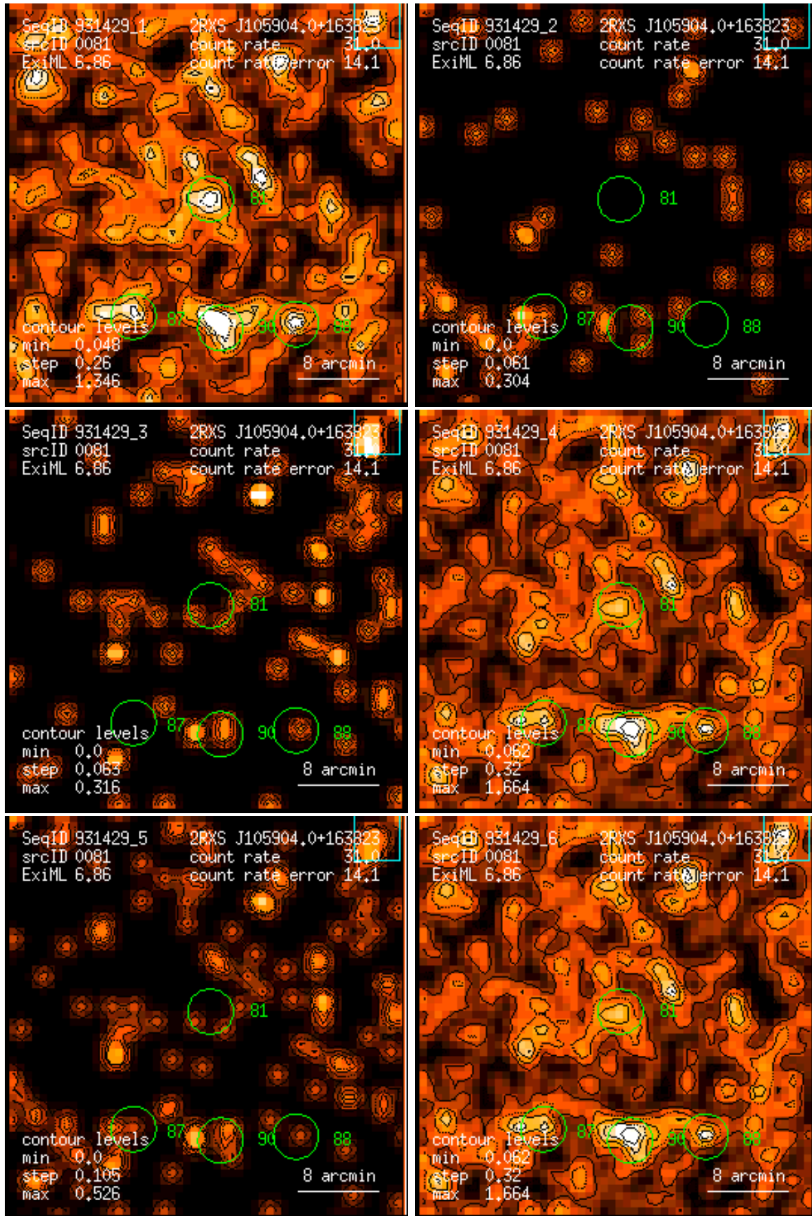
Figure 81: RASS 931429: detection 0081: band rate images, Gaussian filter: (1) PSPC channels 11 – 41, (2) 52 – 90, (3) 91 – 201, (4) 11 – 235, (5) 52 – 201, (6) 11 – 201. Broad band rates in counts/ks. Band rate contour levels in counts/ks/arcmin 2 .
