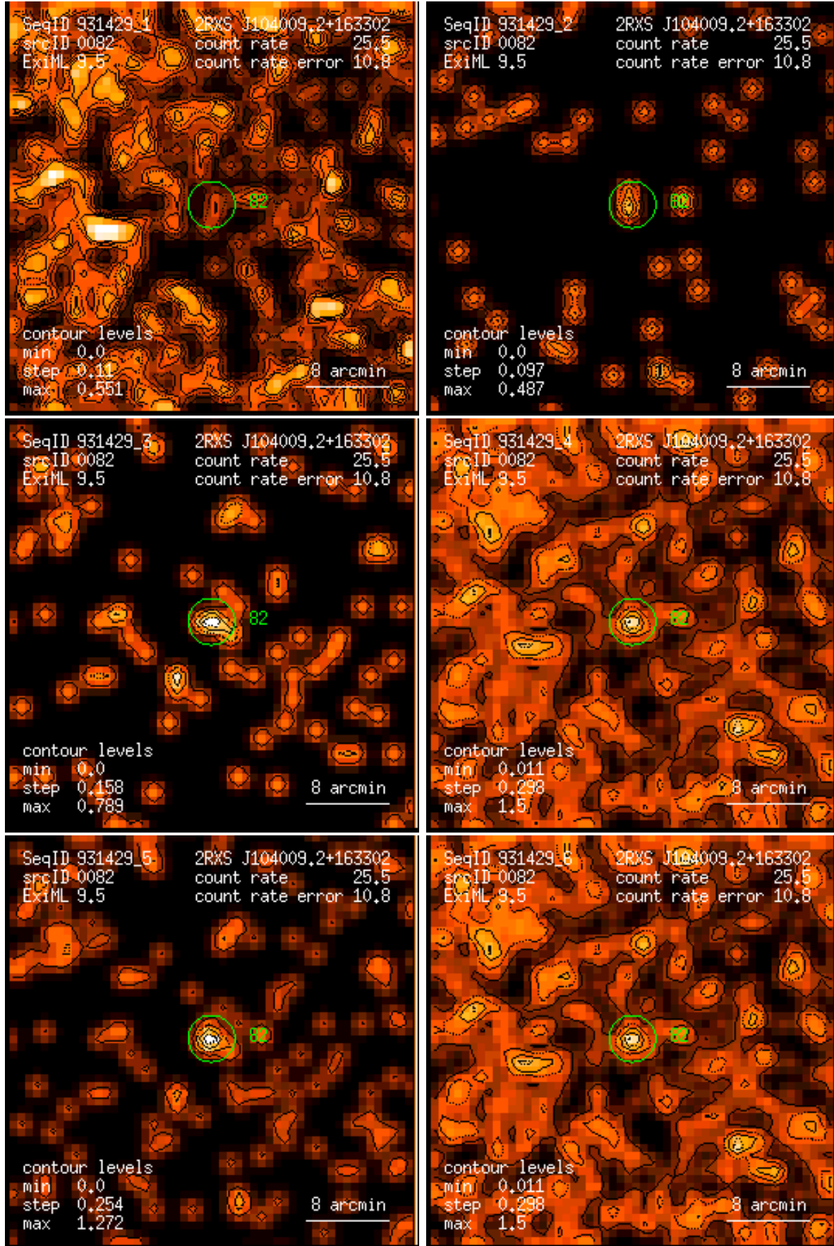
Figure 82: RASS 931429: detection 0082: band rate images, Gaussian filter: (1) PSPC channels 11 – 41, (2) 52 – 90, (3) 91 – 201, (4) 11 – 235, (5) 52 – 201, (6) 11 – 201. Broad band rates in counts/ks. Band rate contour levels in counts/ks/arcmin 2 .
