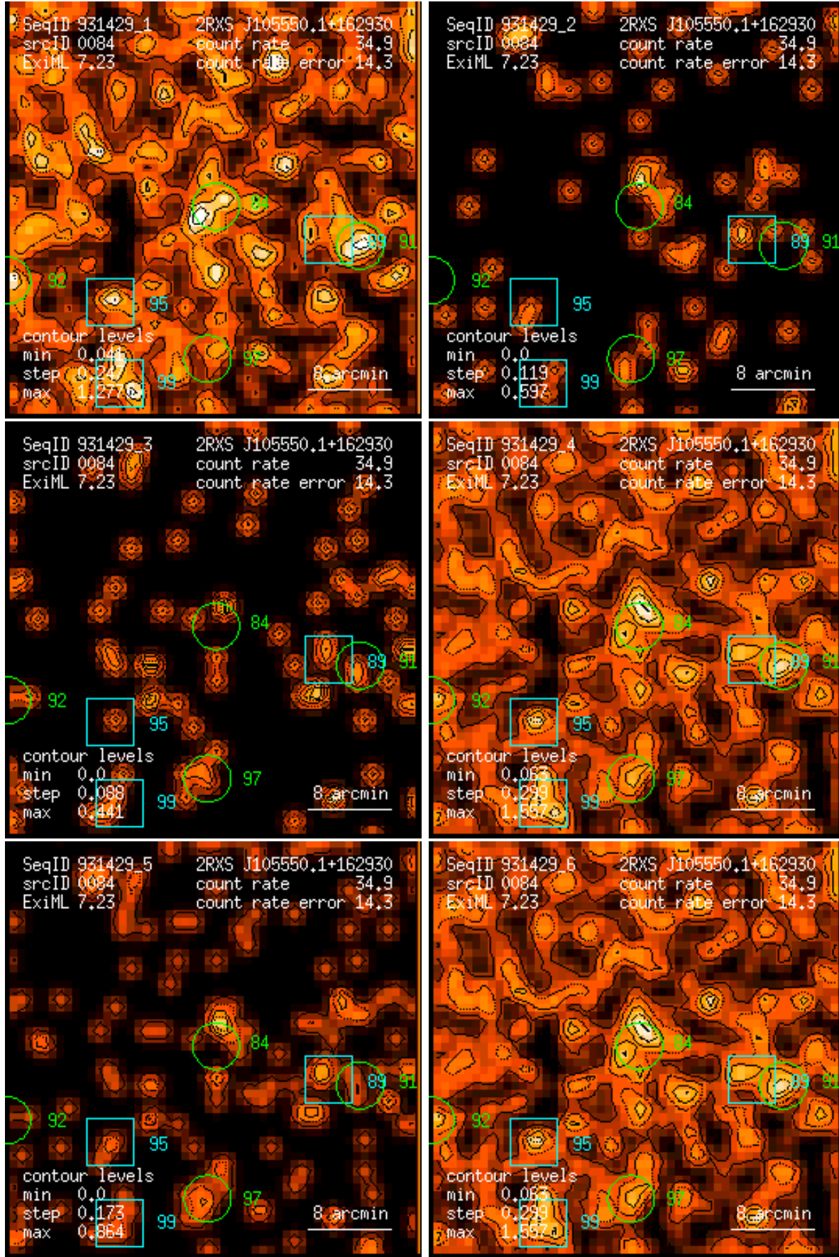
Figure 84: RASS 931429: detection 0084: band rate images, Gaussian filter: (1) PSPC channels 11 – 41, (2) 52 – 90, (3) 91 – 201, (4) 11 – 235, (5) 52 – 201, (6) 11 – 201. Broad band rates in counts/ks. Band rate contour levels in counts/ks/arcmin 2 .
