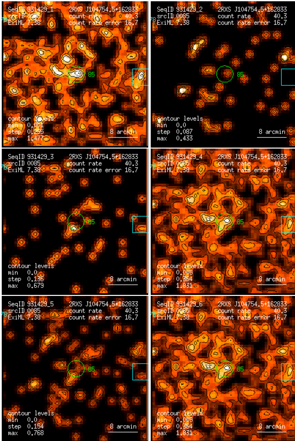
Figure 85: RASS 931429: detection 0085: band rate images, Gaussian filter: (1) PSPC channels 11 – 41, (2) 52 – 90, (3) 91 – 201, (4) 11 – 235, (5) 52 – 201, (6) 11 – 201. Broad band rates in counts/ks. Band rate contour levels in counts/ks/arcmin 2 .
