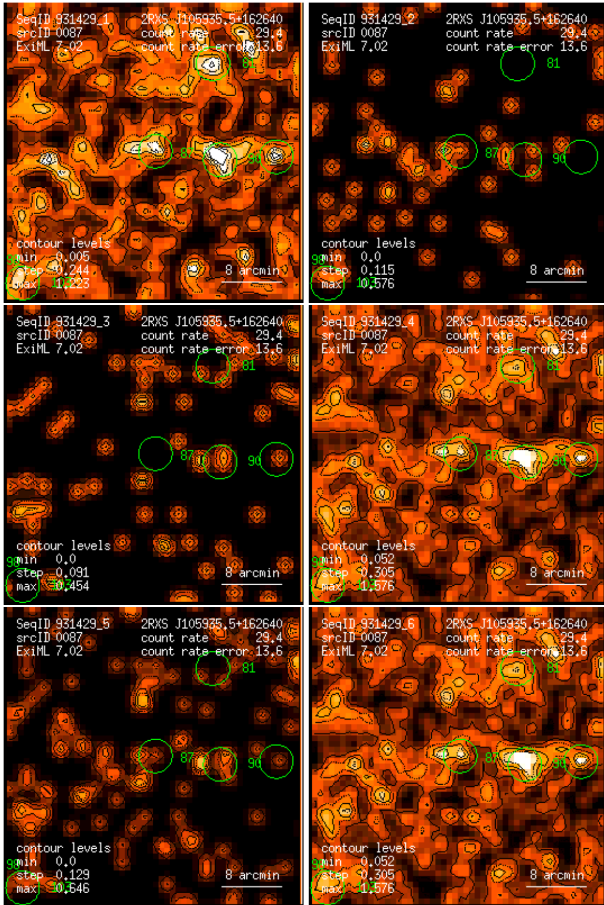
Figure 87: RASS 931429: detection 0087: band rate images, Gaussian filter: (1) PSPC channels 11 – 41, (2) 52 – 90, (3) 91 – 201, (4) 11 – 235, (5) 52 – 201, (6) 11 – 201. Broad band rates in counts/ks. Band rate contour levels in counts/ks/arcmin 2 .
