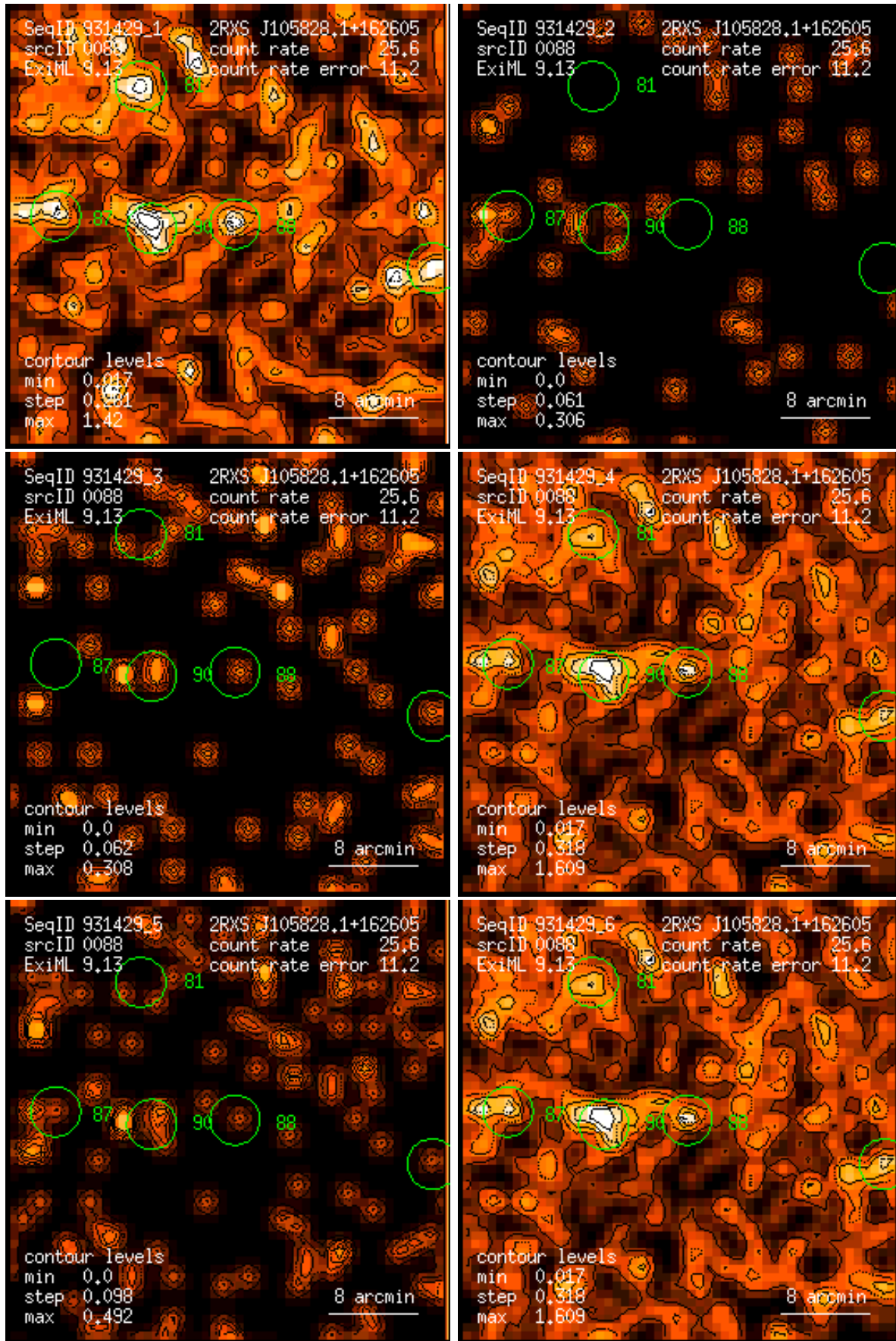
Figure 88: RASS 931429: detection 0088: band rate images, Gaussian filter: (1) PSPC channels 11 – 41, (2) 52 – 90, (3) 91 – 201, (4) 11 – 235, (5) 52 – 201, (6) 11 – 201. Broad band rates in counts/ks. Band rate contour levels in counts/ks/arcmin 2 .
