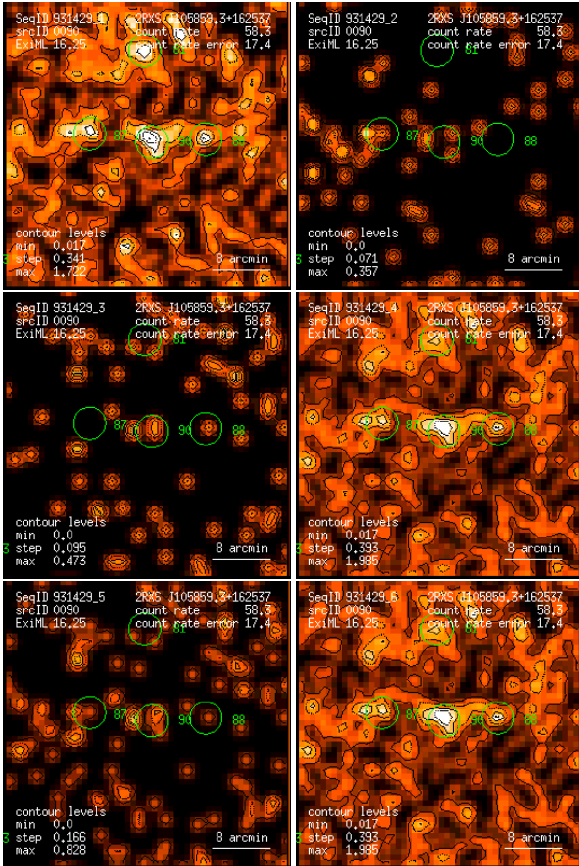
Figure 90: RASS 931429: detection 0090: band rate images, Gaussian filter: (1) PSPC channels 11 – 41, (2) 52 – 90, (3) 91 – 201, (4) 11 – 235, (5) 52 – 201, (6) 11 – 201. Broad band rates in counts/ks. Band rate contour levels in counts/ks/arcmin 2 .
