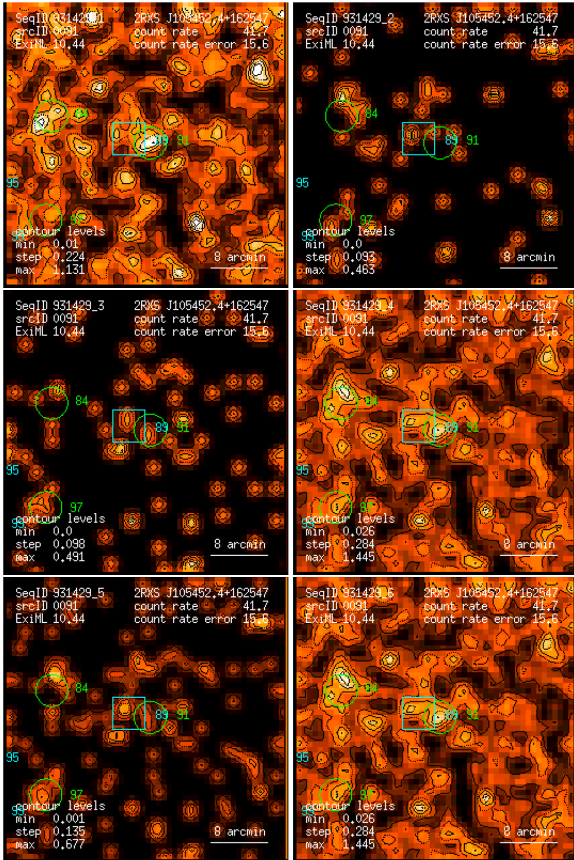
Figure 91: RASS 931429: detection 0091: band rate images, Gaussian filter: (1) PSPC channels 11 – 41, (2) 52 – 90, (3) 91 – 201, (4) 11 – 235, (5) 52 – 201, (6) 11 – 201. Broad band rates in counts/ks. Band rate contour levels in counts/ks/arcmin 2 .
