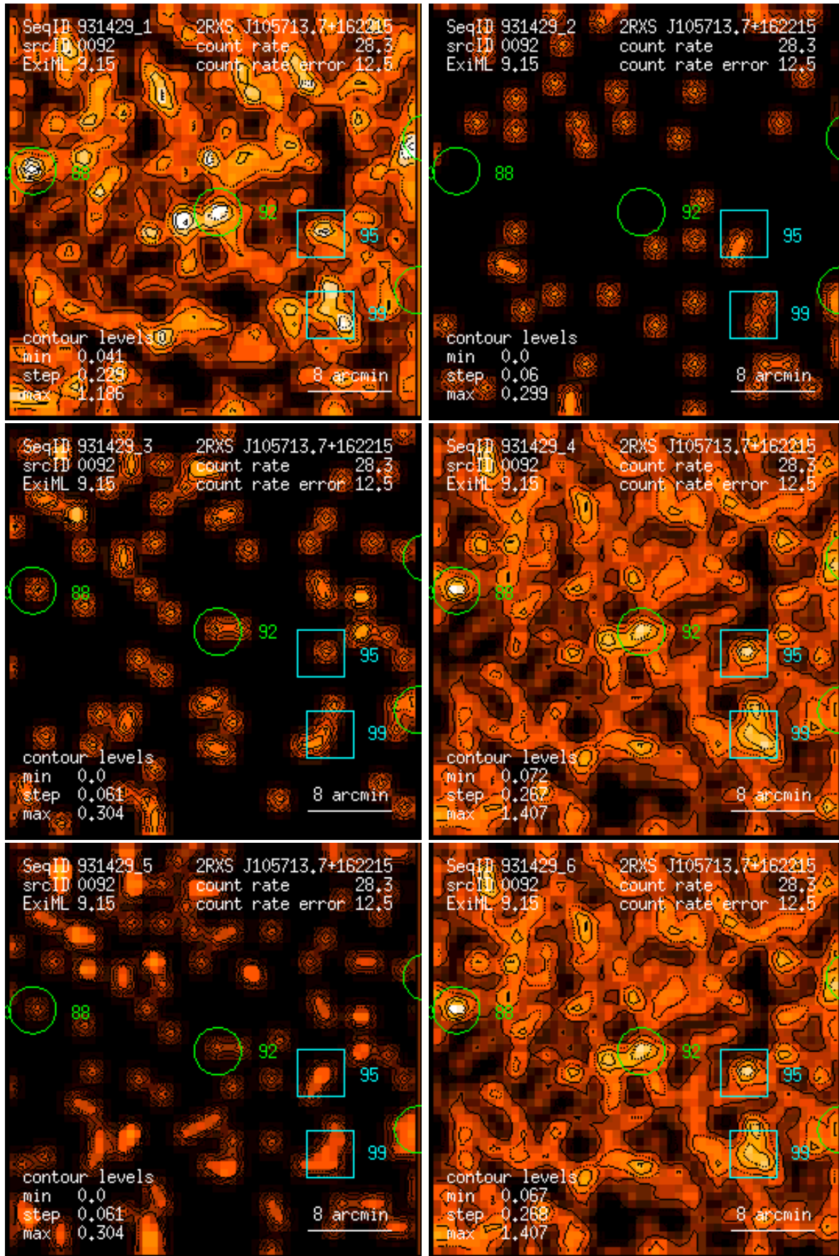
Figure 92: RASS 931429: detection 0092: band rate images, Gaussian filter: (1) PSPC channels 11 – 41, (2) 52 – 90, (3) 91 – 201, (4) 11 – 235, (5) 52 – 201, (6) 11 – 201. Broad band rates in counts/ks. Band rate contour levels in counts/ks/arcmin 2 .
