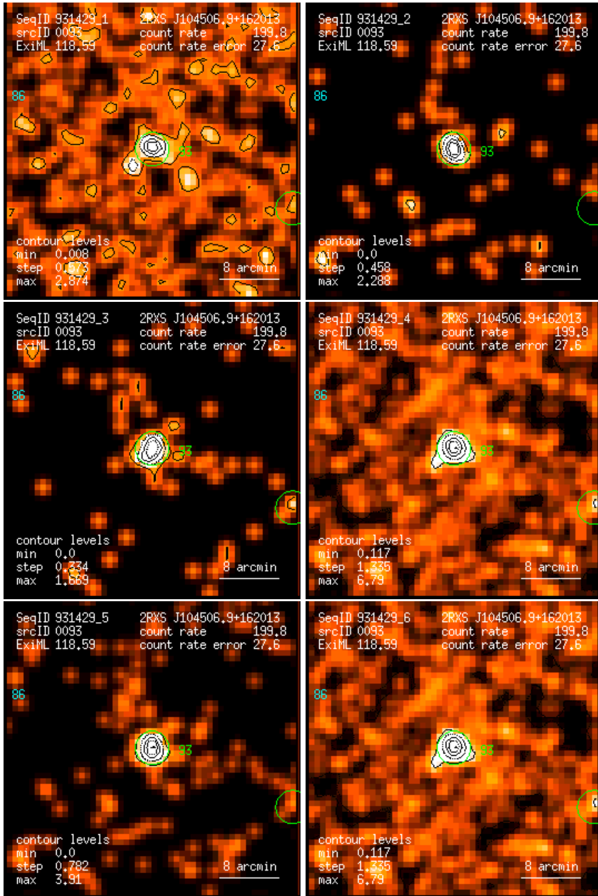
Figure 93: RASS 931429: detection 0093: band rate images, Gaussian filter: (1) PSPC channels 11 – 41, (2) 52 – 90, (3) 91 – 201, (4) 11 – 235, (5) 52 – 201, (6) 11 – 201. Broad band rates in counts/ks. Band rate contour levels in counts/ks/arcmin 2 .
