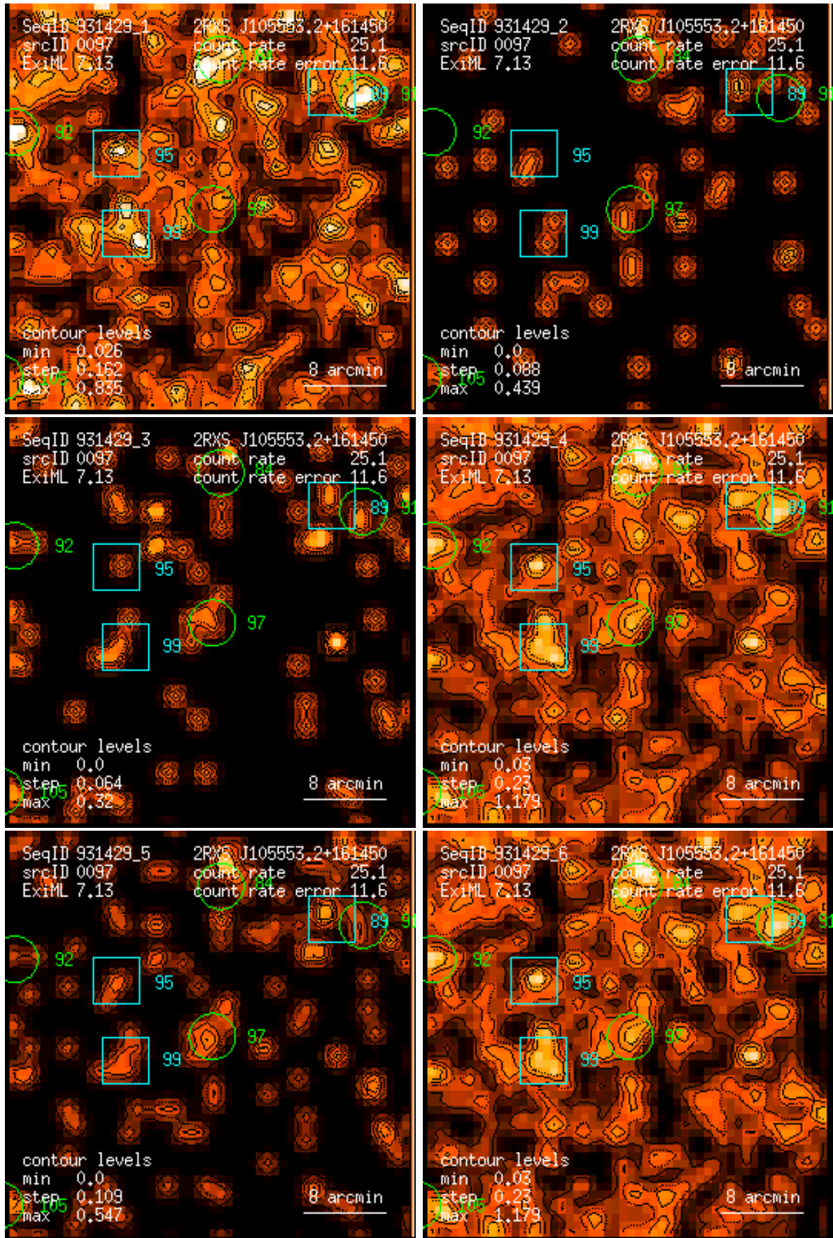
Figure 97: RASS 931429: detection 0097: band rate images, Gaussian filter: (1) PSPC channels 11 – 41, (2) 52 – 90, (3) 91 – 201, (4) 11 – 235, (5) 52 – 201, (6) 11 – 201. Broad band rates in counts/ks. Band rate contour levels in counts/ks/arcmin 2 .
