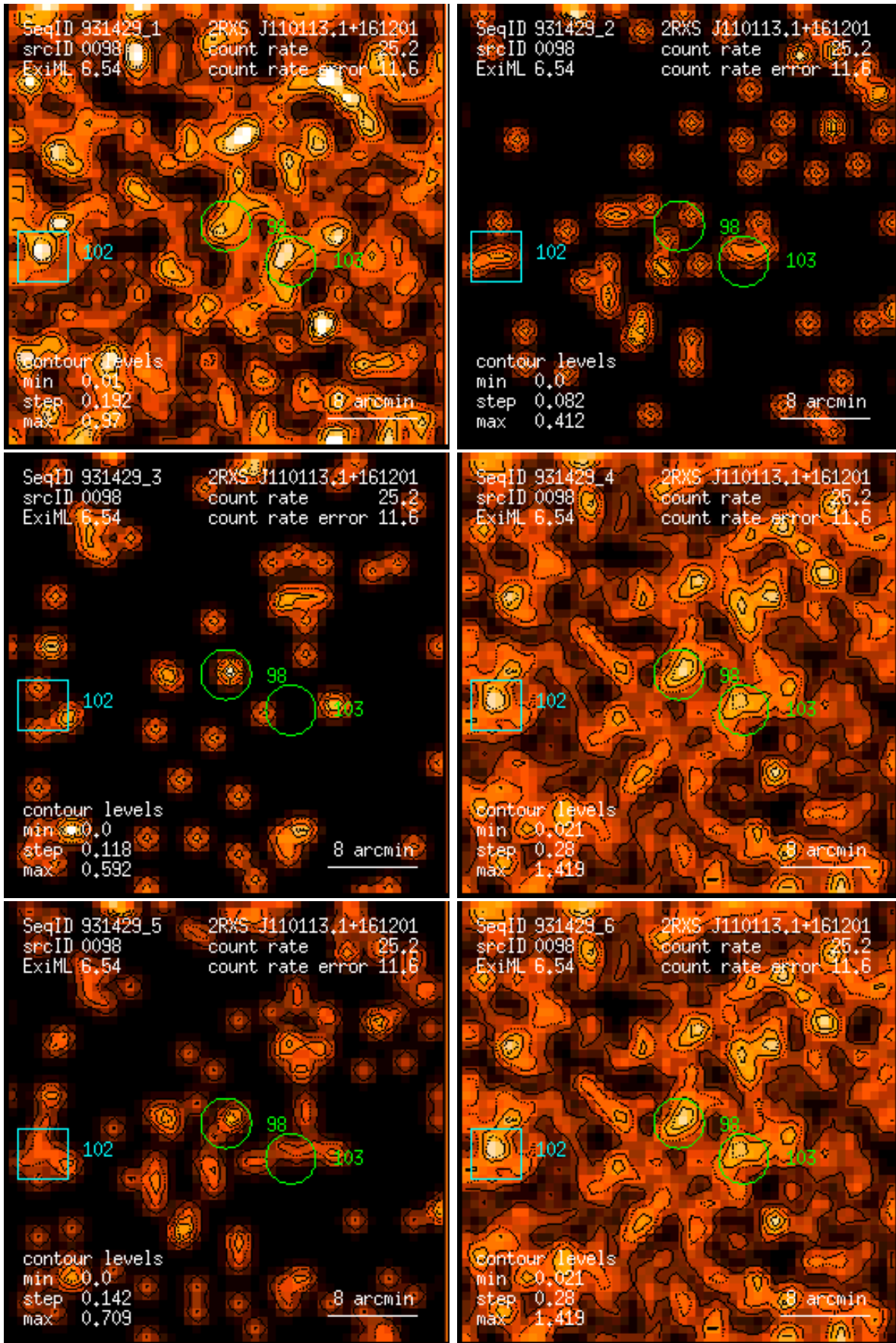
Figure 98: RASS 931429: detection 0098: band rate images, Gaussian filter: (1) PSPC channels 11 – 41, (2) 52 – 90, (3) 91 – 201, (4) 11 – 235, (5) 52 – 201, (6) 11 – 201. Broad band rates in counts/ks. Band rate contour levels in counts/ks/arcmin 2 .
