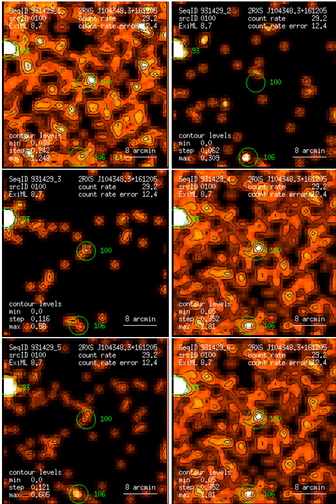
Figure 100: RASS 931429: detection 0100: band rate images, Gaussian filter: (1) PSPC channels 11 – 41, (2) 52 – 90, (3) 91 – 201, (4) 11 – 235, (5) 52 – 201, (6) 11 – 201. Broad band rates in counts/ks. Band rate contour levels in counts/ks/arcmin 2 .
