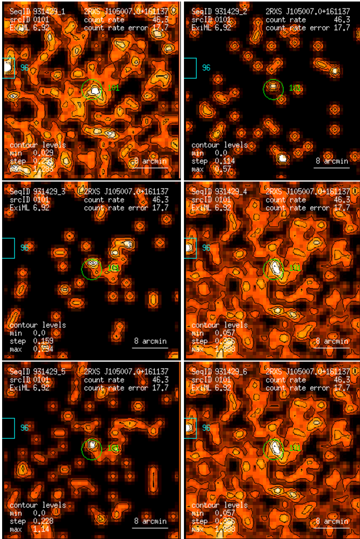
Figure 101: RASS 931429: detection 0101: band rate images, Gaussian filter: (1) PSPC channels 11 – 41, (2) 52 – 90, (3) 91 – 201, (4) 11 – 235, (5) 52 – 201, (6) 11 – 201. Broad band rates in counts/ks. Band rate contour levels in counts/ks/arcmin 2 .
