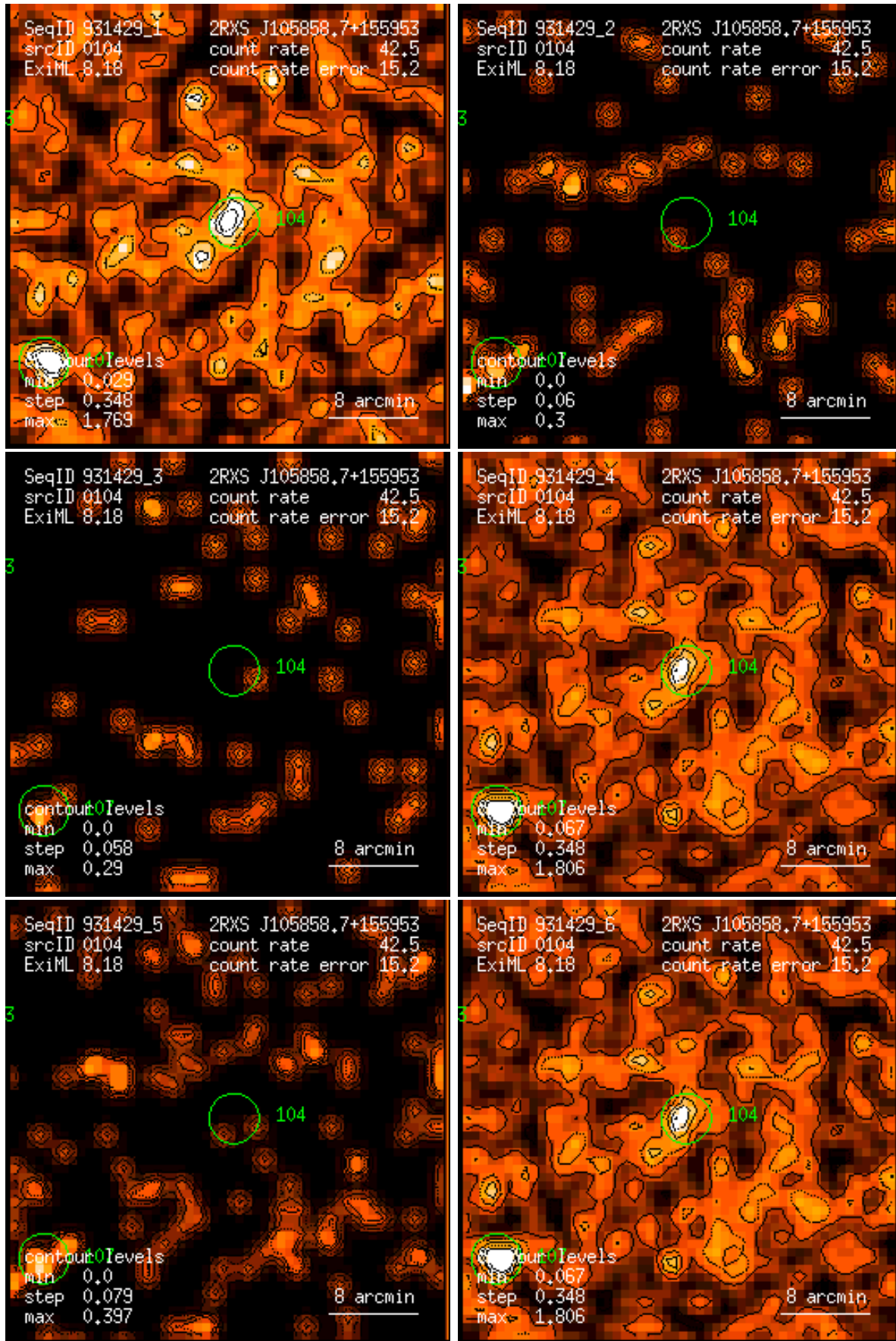
Figure 104: RASS 931429: detection 0104: band rate images, Gaussian filter: (1) PSPC channels 11 – 41, (2) 52 – 90, (3) 91 – 201, (4) 11 – 235, (5) 52 – 201, (6) 11 – 201. Broad band rates in counts/ks. Band rate contour levels in counts/ks/arcmin 2 .
