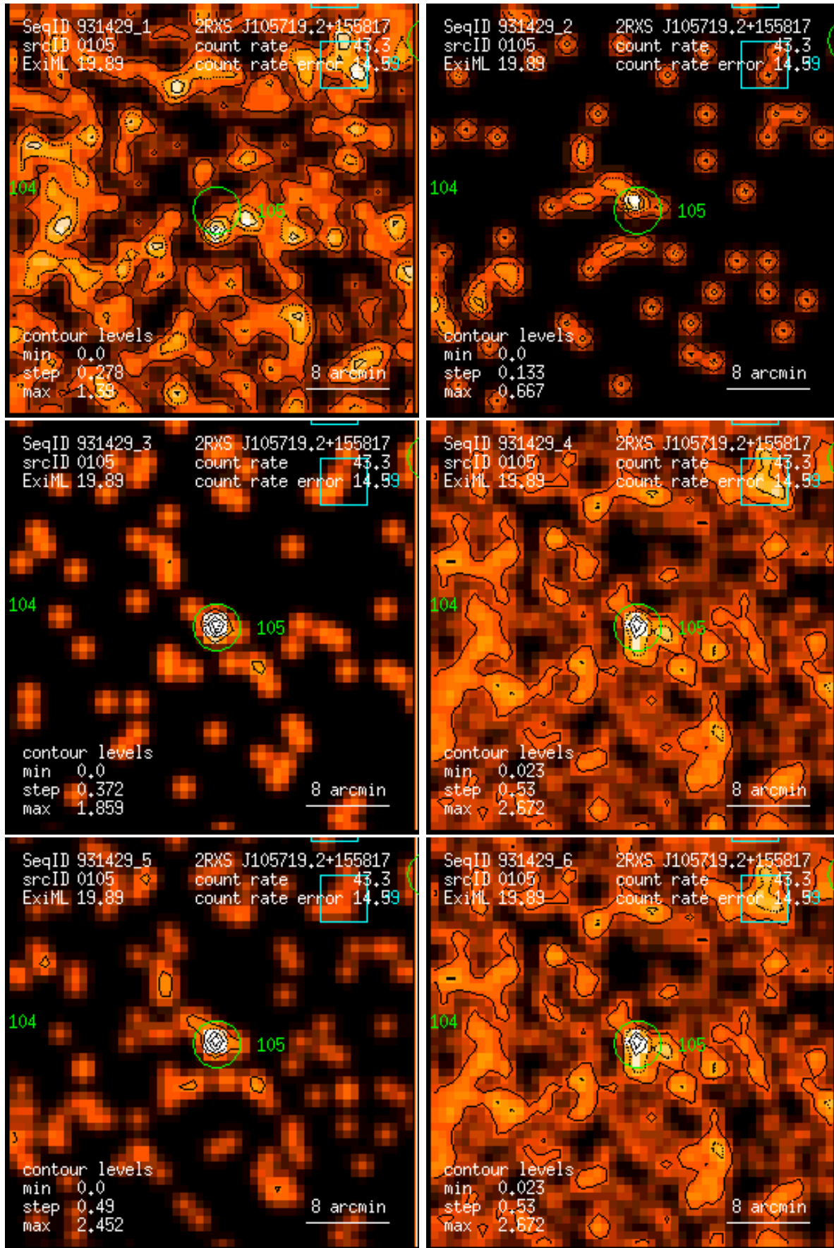
Figure 105: RASS 931429: detection 0105: band rate images, Gaussian filter: (1) PSPC channels 11 – 41, (2) 52 – 90, (3) 91 – 201, (4) 11 – 235, (5) 52 – 201, (6) 11 – 201. Broad band rates in counts/ks. Band rate contour levels in counts/ks/arcmin 2 .
