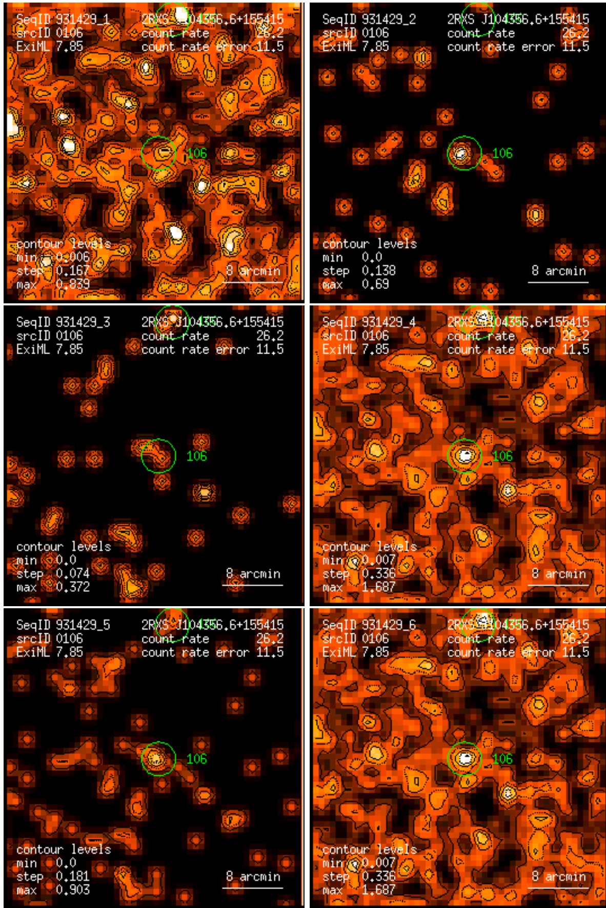
Figure 106: RASS 931429: detection 0106: band rate images, Gaussian filter: (1) PSPC channels 11 – 41, (2) 52 – 90, (3) 91 – 201, (4) 11 – 235, (5) 52 – 201, (6) 11 – 201. Broad band rates in counts/ks. Band rate contour levels in counts/ks/arcmin 2 .
