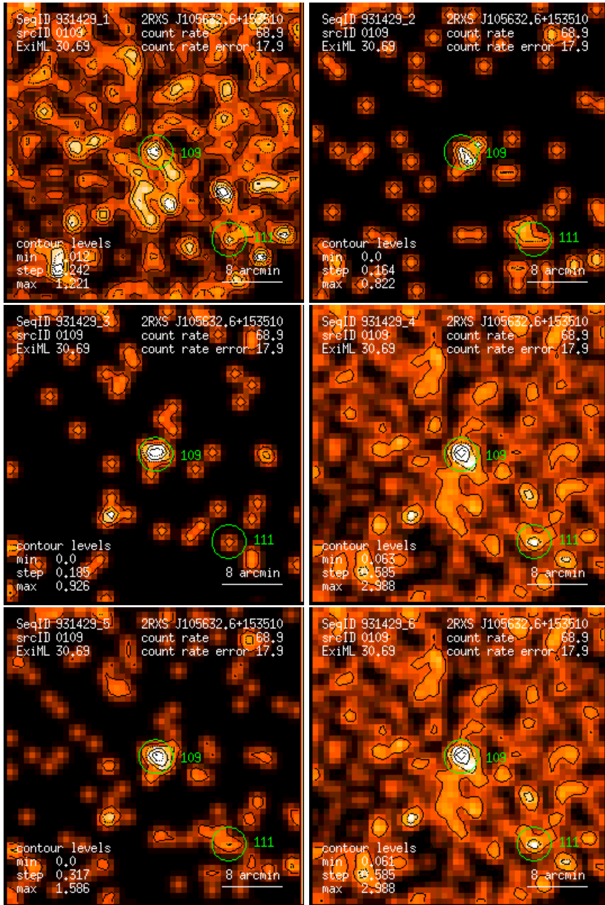
Figure 109: RASS 931429: detection 0109: band rate images, Gaussian filter: (1) PSPC channels 11 – 41, (2) 52 – 90, (3) 91 – 201, (4) 11 – 235, (5) 52 – 201, (6) 11 – 201. Broad band rates in counts/ks. Band rate contour levels in counts/ks/arcmin 2 .
