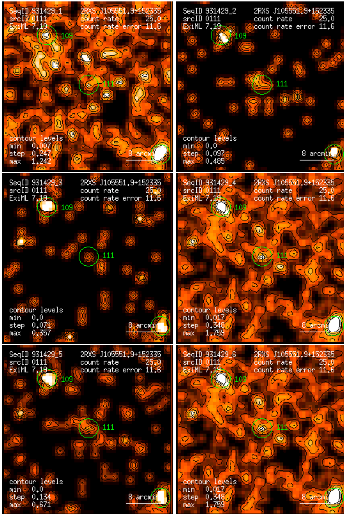
Figure 111: RASS 931429: detection 0111: band rate images, Gaussian filter: (1) PSPC channels 11 – 41, (2) 52 – 90, (3) 91 – 201, (4) 11 – 235, (5) 52 – 201, (6) 11 – 201. Broad band rates in counts/ks. Band rate contour levels in counts/ks/arcmin 2 .
