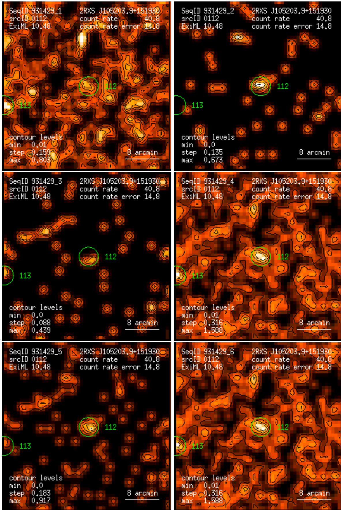
Figure 112: RASS 931429: detection 0112: band rate images, Gaussian filter: (1) PSPC channels 11 – 41, (2) 52 – 90, (3) 91 – 201, (4) 11 – 235, (5) 52 – 201, (6) 11 – 201. Broad band rates in counts/ks. Band rate contour levels in counts/ks/arcmin 2 .
