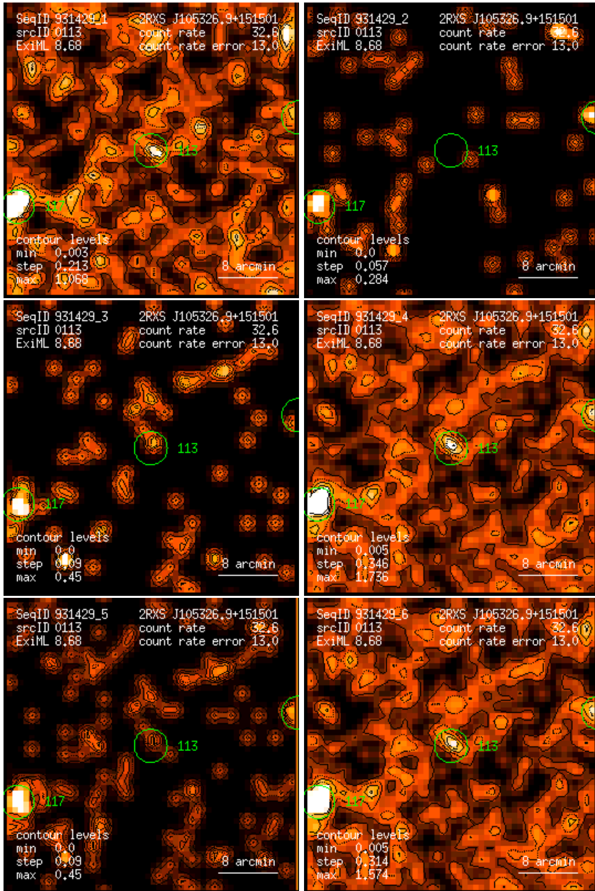
Figure 113: RASS 931429: detection 0113: band rate images, Gaussian filter: (1) PSPC channels 11 – 41, (2) 52 – 90, (3) 91 – 201, (4) 11 – 235, (5) 52 – 201, (6) 11 – 201. Broad band rates in counts/ks. Band rate contour levels in counts/ks/arcmin 2 .
