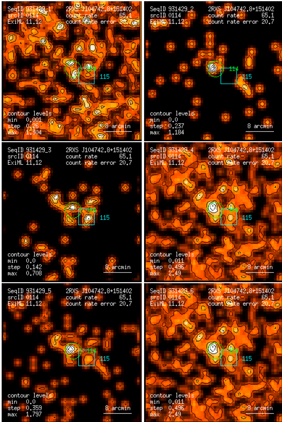
Figure 114: RASS 931429: detection 0114: band rate images, Gaussian filter: (1) PSPC channels 11 – 41, (2) 52 – 90, (3) 91 – 201, (4) 11 – 235, (5) 52 – 201, (6) 11 – 201. Broad band rates in counts/ks. Band rate contour levels in counts/ks/arcmin 2 .
