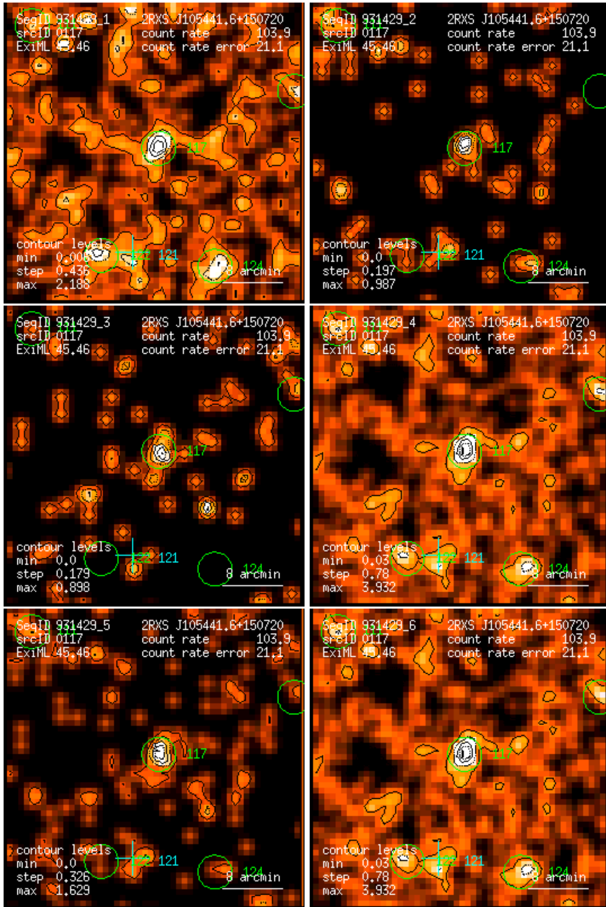
Figure 117: RASS 931429: detection 0117: band rate images, Gaussian filter: (1) PSPC channels 11 – 41, (2) 52 – 90, (3) 91 – 201, (4) 11 – 235, (5) 52 – 201, (6) 11 – 201. Broad band rates in counts/ks. Band rate contour levels in counts/ks/arcmin 2 .
