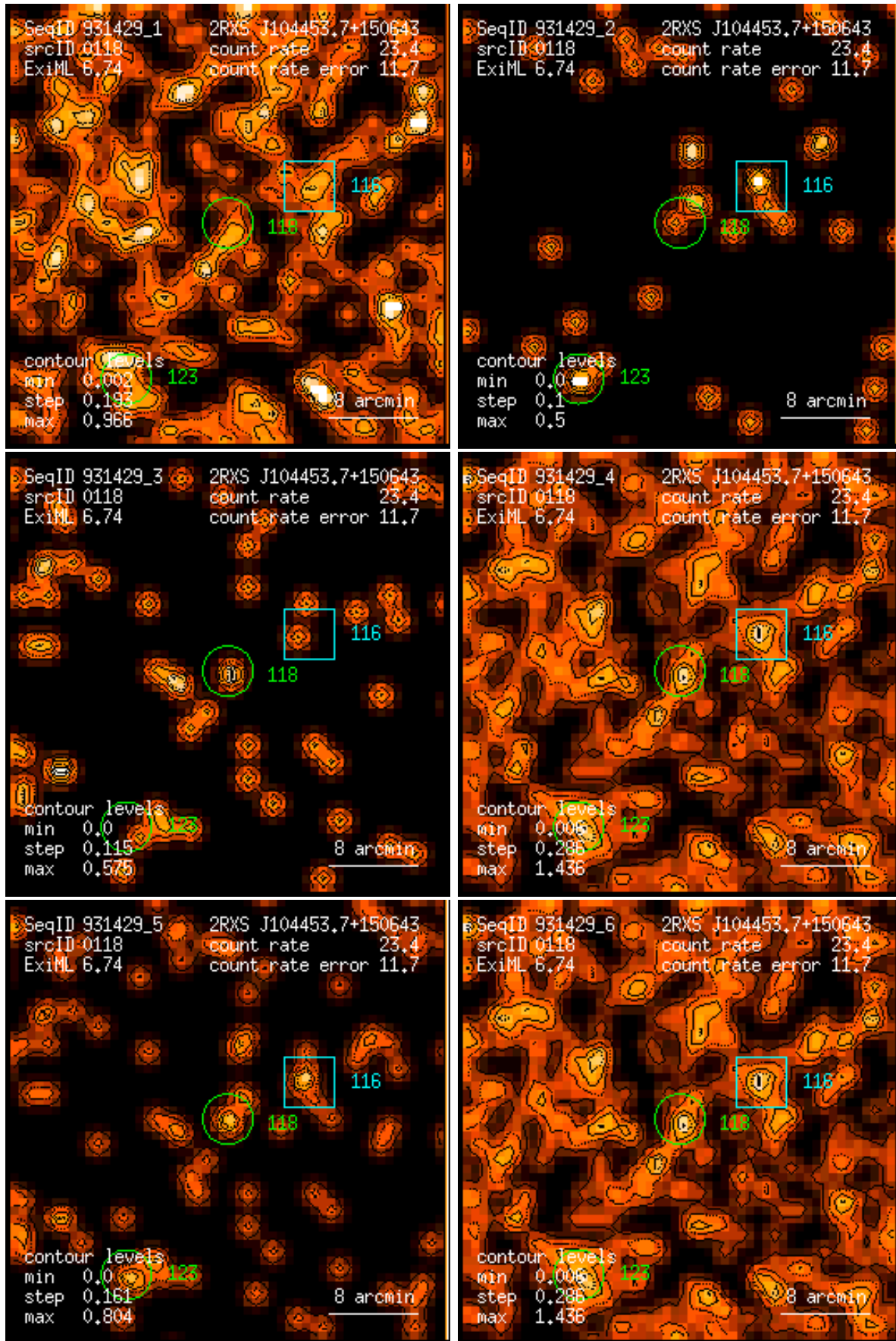
Figure 118: RASS 931429: detection 0118: band rate images, Gaussian filter: (1) PSPC channels 11 – 41, (2) 52 – 90, (3) 91 – 201, (4) 11 – 235, (5) 52 – 201, (6) 11 – 201. Broad band rates in counts/ks. Band rate contour levels in counts/ks/arcmin 2 .
