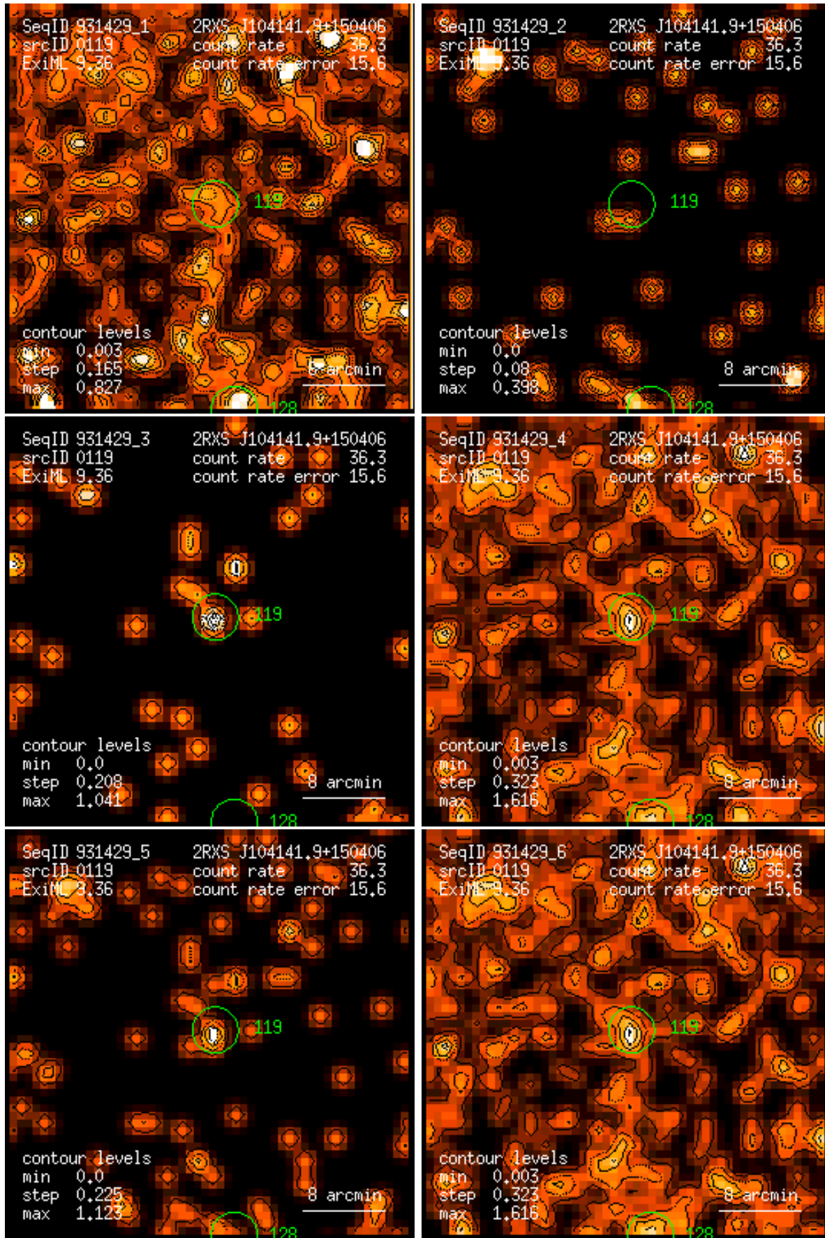
Figure 119: RASS 931429: detection 0119: band rate images, Gaussian filter: (1) PSPC channels 11 – 41, (2) 52 – 90, (3) 91 – 201, (4) 11 – 235, (5) 52 – 201, (6) 11 – 201. Broad band rates in counts/ks. Band rate contour levels in counts/ks/arcmin 2 .
