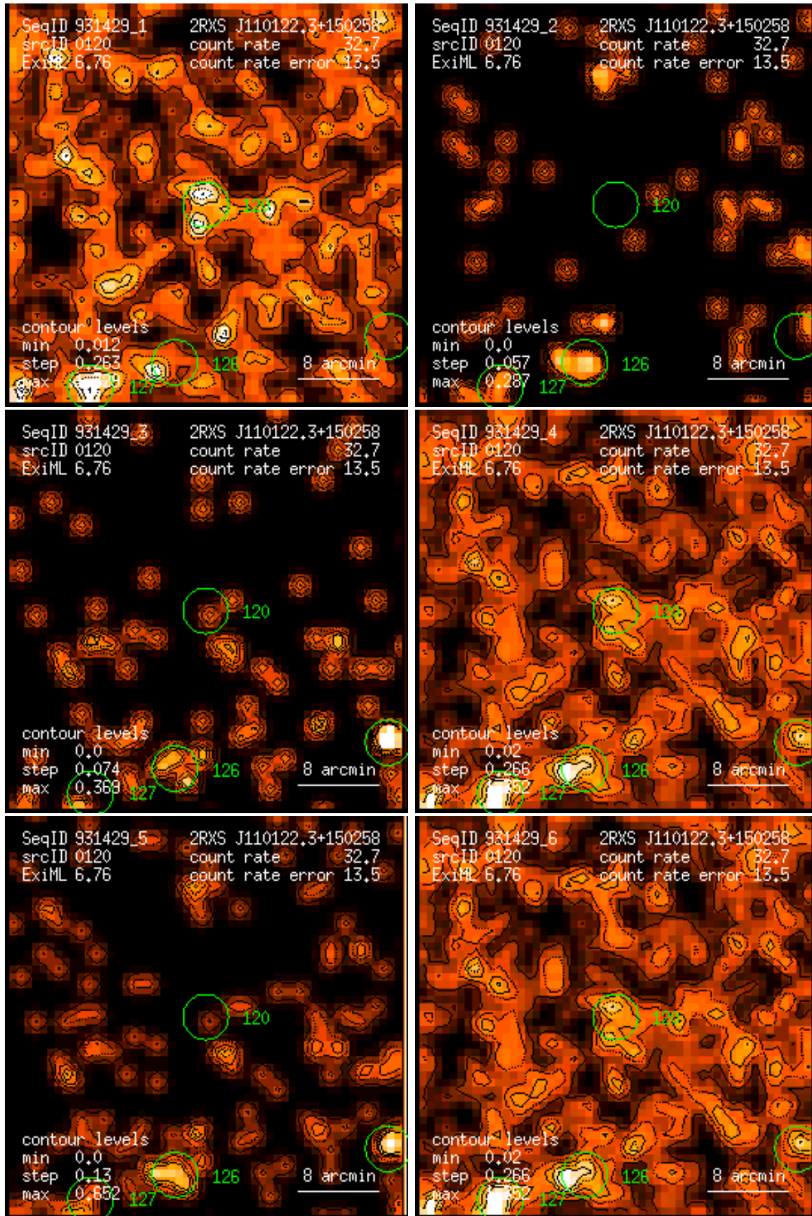
Figure 120: RASS 931429: detection 0120: band rate images, Gaussian filter: (1) PSPC channels 11 – 41, (2) 52 – 90, (3) 91 – 201, (4) 11 – 235, (5) 52 – 201, (6) 11 – 201. Broad band rates in counts/ks. Band rate contour levels in counts/ks/arcmin 2 .
