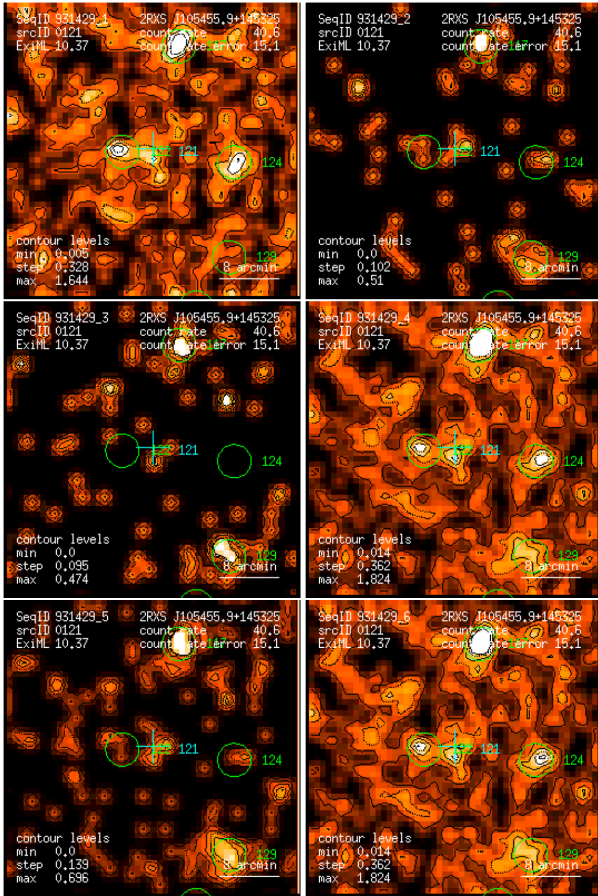
Figure 121: RASS 931429: detection 0121: band rate images, Gaussian filter: (1) PSPC channels 11 – 41, (2) 52 – 90, (3) 91 – 201, (4) 11 – 235, (5) 52 – 201, (6) 11 – 201. Broad band rates in counts/ks. Band rate contour levels in counts/ks/arcmin 2 .
