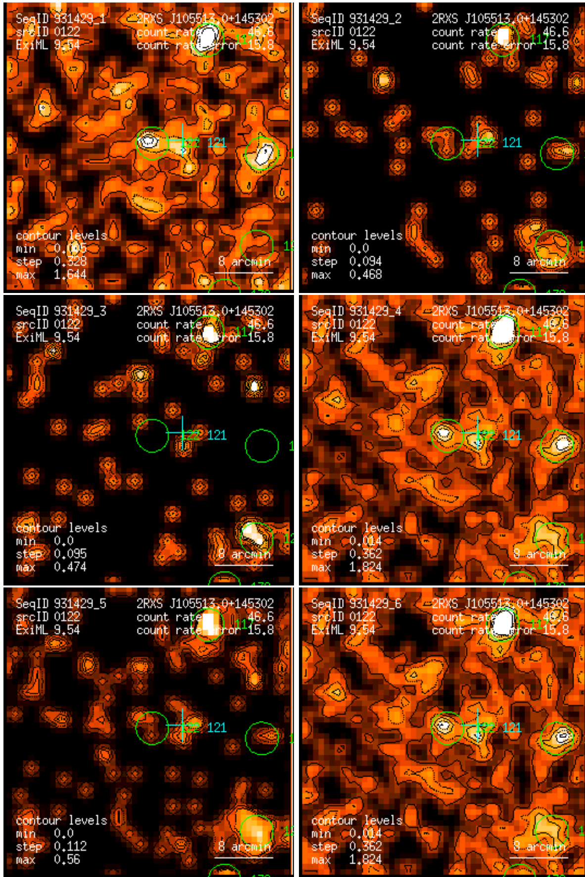
Figure 122: RASS 931429: detection 0122: band rate images, Gaussian filter: (1) PSPC channels 11 – 41, (2) 52 – 90, (3) 91 – 201, (4) 11 – 235, (5) 52 – 201, (6) 11 – 201. Broad band rates in counts/ks. Band rate contour levels in counts/ks/arcmin 2 .
