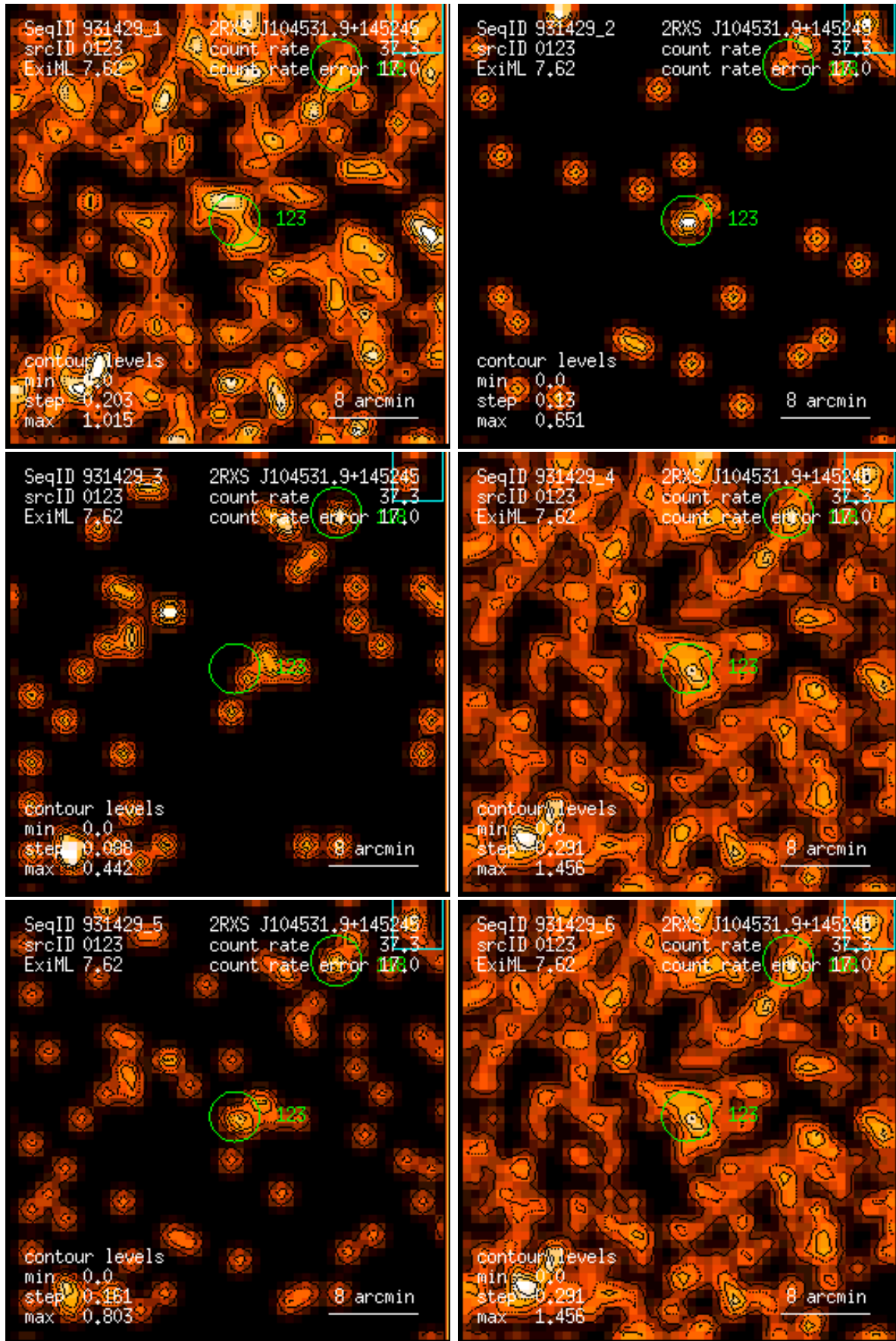
Figure 123: RASS 931429: detection 0123: band rate images, Gaussian filter: (1) PSPC channels 11 – 41, (2) 52 – 90, (3) 91 – 201, (4) 11 – 235, (5) 52 – 201, (6) 11 – 201. Broad band rates in counts/ks. Band rate contour levels in counts/ks/arcmin 2 .
