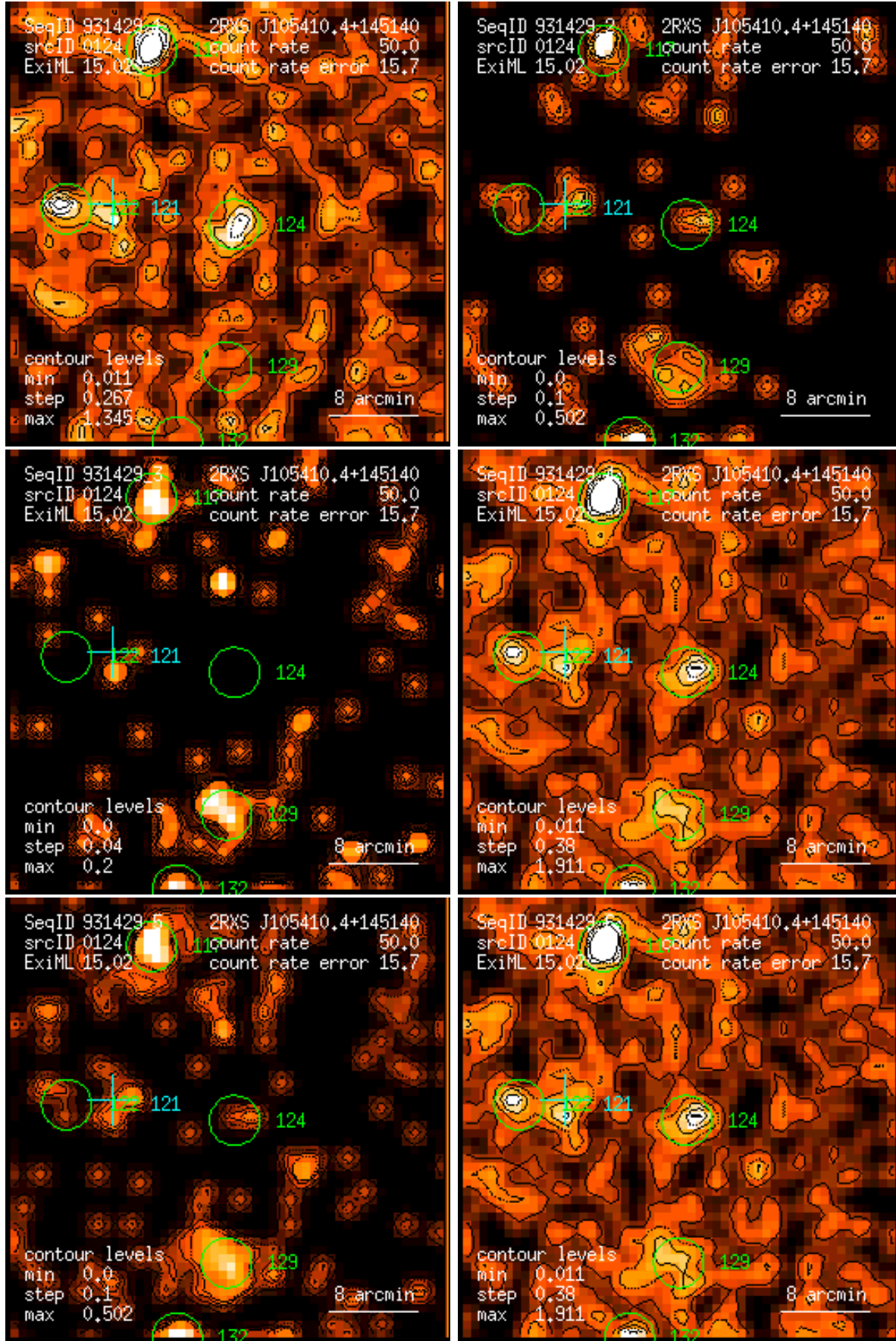
Figure 124: RASS 931429: detection 0124: band rate images, Gaussian filter: (1) PSPC channels 11 – 41, (2) 52 – 90, (3) 91 – 201, (4) 11 – 235, (5) 52 – 201, (6) 11 – 201. Broad band rates in counts/ks. Band rate contour levels in counts/ks/arcmin 2 .
