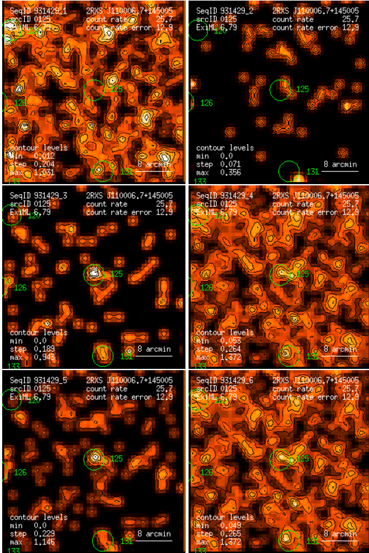
Figure 125: RASS 931429: detection 0125: band rate images, Gaussian filter: (1) PSPC channels 11 – 41, (2) 52 – 90, (3) 91 – 201, (4) 11 – 235, (5) 52 – 201, (6) 11 – 201. Broad band rates in counts/ks. Band rate contour levels in counts/ks/arcmin 2 .
