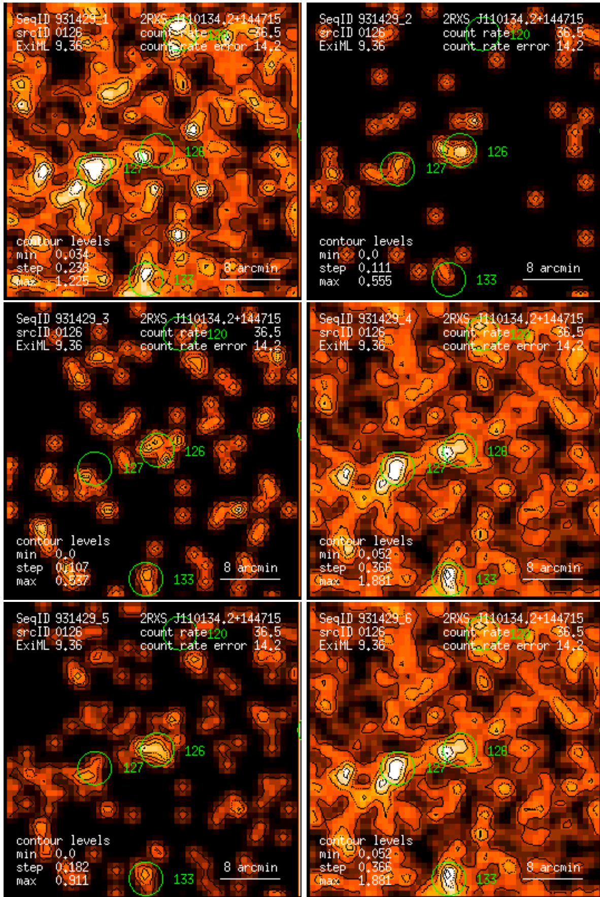
Figure 126: RASS 931429: detection 0126: band rate images, Gaussian filter: (1) PSPC channels 11 – 41, (2) 52 – 90, (3) 91 – 201, (4) 11 – 235, (5) 52 – 201, (6) 11 – 201. Broad band rates in counts/ks. Band rate contour levels in counts/ks/arcmin 2 .
