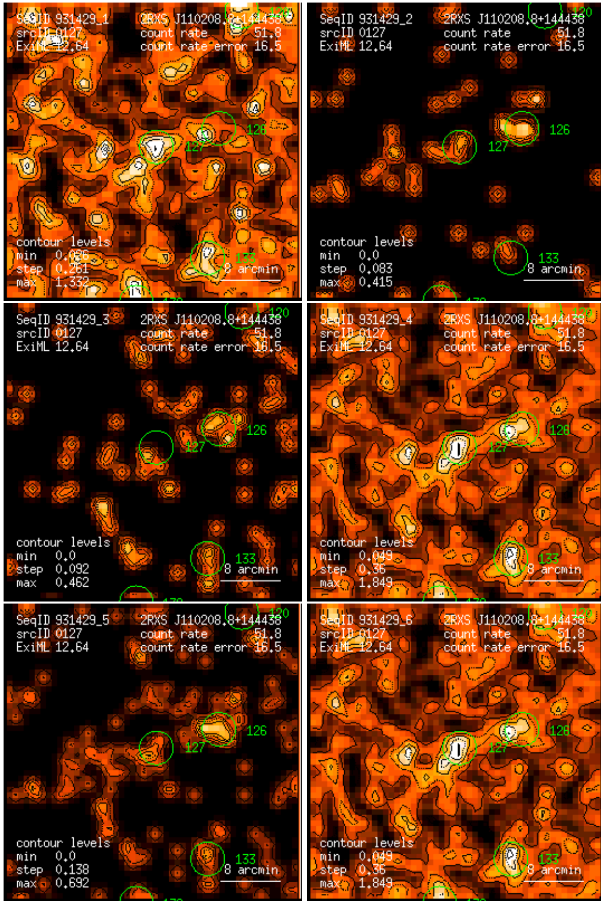
Figure 127: RASS 931429: detection 0127: band rate images, Gaussian filter: (1) PSPC channels 11 – 41, (2) 52 – 90, (3) 91 – 201, (4) 11 – 235, (5) 52 – 201, (6) 11 – 201. Broad band rates in counts/ks. Band rate contour levels in counts/ks/arcmin 2 .
