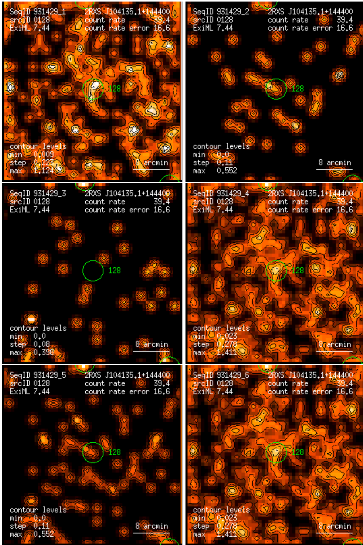
Figure 128: RASS 931429: detection 0128: band rate images, Gaussian filter: (1) PSPC channels 11 – 41, (2) 52 – 90, (3) 91 – 201, (4) 11 – 235, (5) 52 – 201, (6) 11 – 201. Broad band rates in counts/ks. Band rate contour levels in counts/ks/arcmin 2 .
