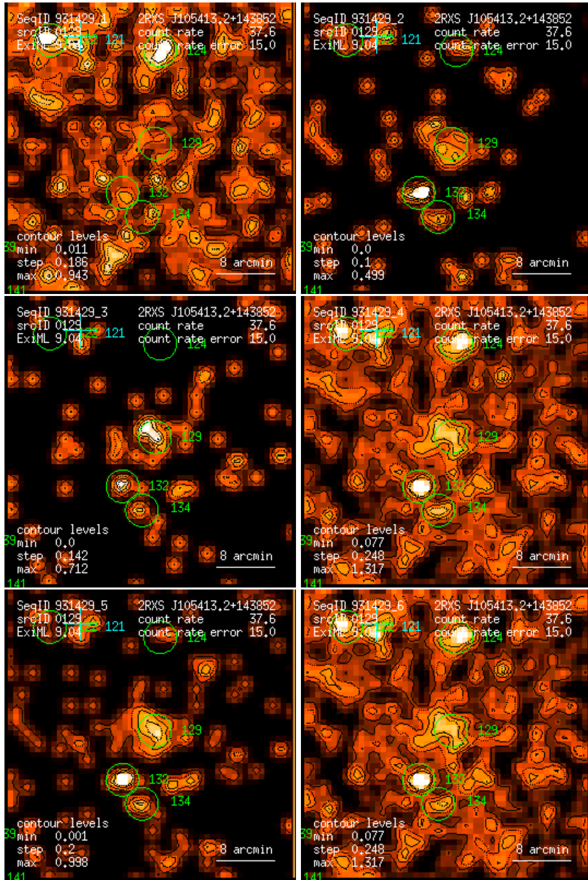
Figure 129: RASS 931429: detection 0129: band rate images, Gaussian filter: (1) PSPC channels 11 – 41, (2) 52 – 90, (3) 91 – 201, (4) 11 – 235, (5) 52 – 201, (6) 11 – 201. Broad band rates in counts/ks. Band rate contour levels in counts/ks/arcmin 2 .
