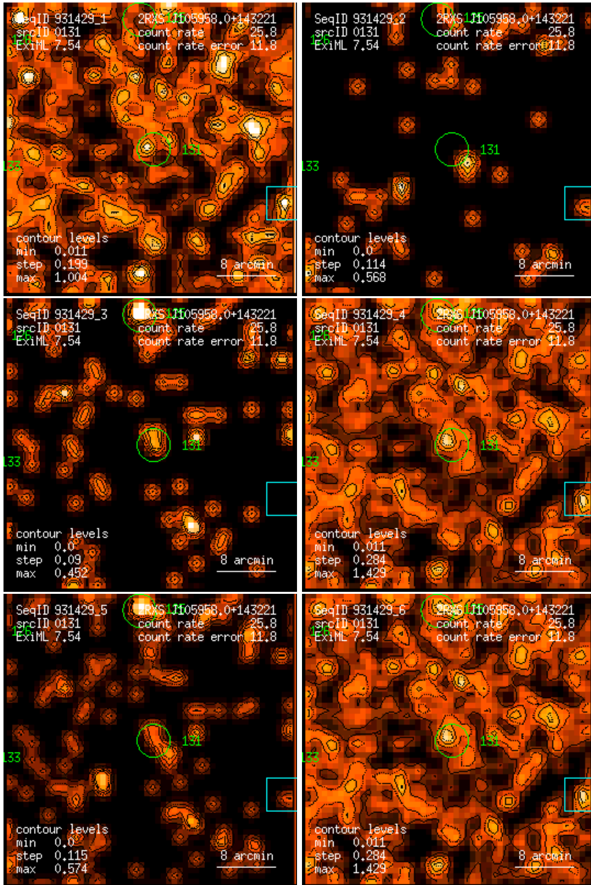
Figure 131: RASS 931429: detection 0131: band rate images, Gaussian filter: (1) PSPC channels 11 – 41, (2) 52 – 90, (3) 91 – 201, (4) 11 – 235, (5) 52 – 201, (6) 11 – 201. Broad band rates in counts/ks. Band rate contour levels in counts/ks/arcmin 2 .
