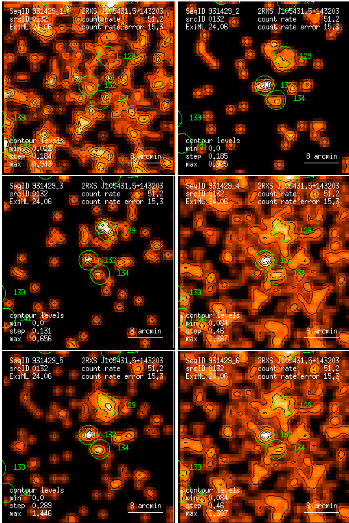
Figure 132: RASS 931429: detection 0132: band rate images, Gaussian filter: (1) PSPC channels 11 – 41, (2) 52 – 90, (3) 91 – 201, (4) 11 – 235, (5) 52 – 201, (6) 11 – 201. Broad band rates in counts/ks. Band rate contour levels in counts/ks/arcmin 2 .
