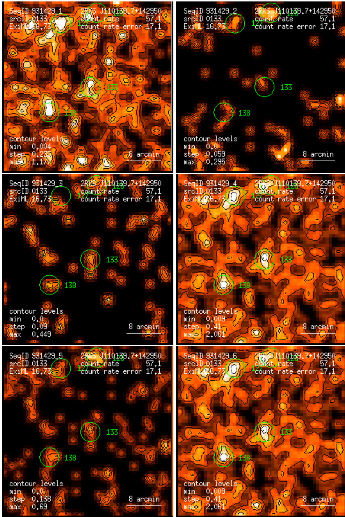
Figure 133: RASS 931429: detection 0133: band rate images, Gaussian filter: (1) PSPC channels 11 – 41, (2) 52 – 90, (3) 91 – 201, (4) 11 – 235, (5) 52 – 201, (6) 11 – 201. Broad band rates in counts/ks. Band rate contour levels in counts/ks/arcmin 2 .
