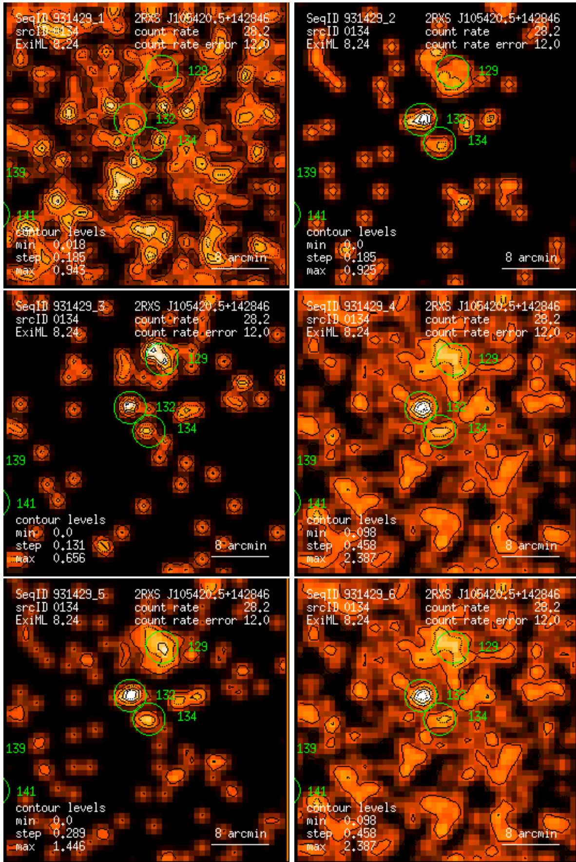
Figure 134: RASS 931429: detection 0134: band rate images, Gaussian filter: (1) PSPC channels 11 – 41, (2) 52 – 90, (3) 91 – 201, (4) 11 – 235, (5) 52 – 201, (6) 11 – 201. Broad band rates in counts/ks. Band rate contour levels in counts/ks/arcmin 2 .
