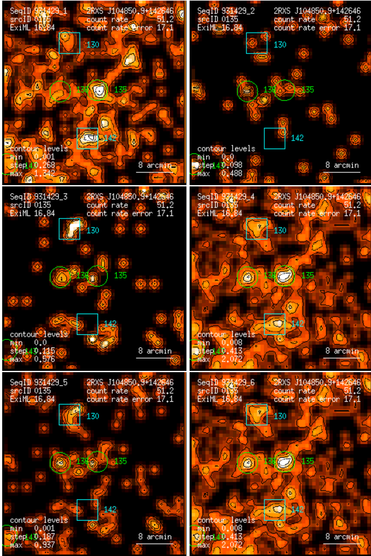
Figure 135: RASS 931429: detection 0135: band rate images, Gaussian filter: (1) PSPC channels 11 – 41, (2) 52 – 90, (3) 91 – 201, (4) 11 – 235, (5) 52 – 201, (6) 11 – 201. Broad band rates in counts/ks. Band rate contour levels in counts/ks/arcmin 2 .
