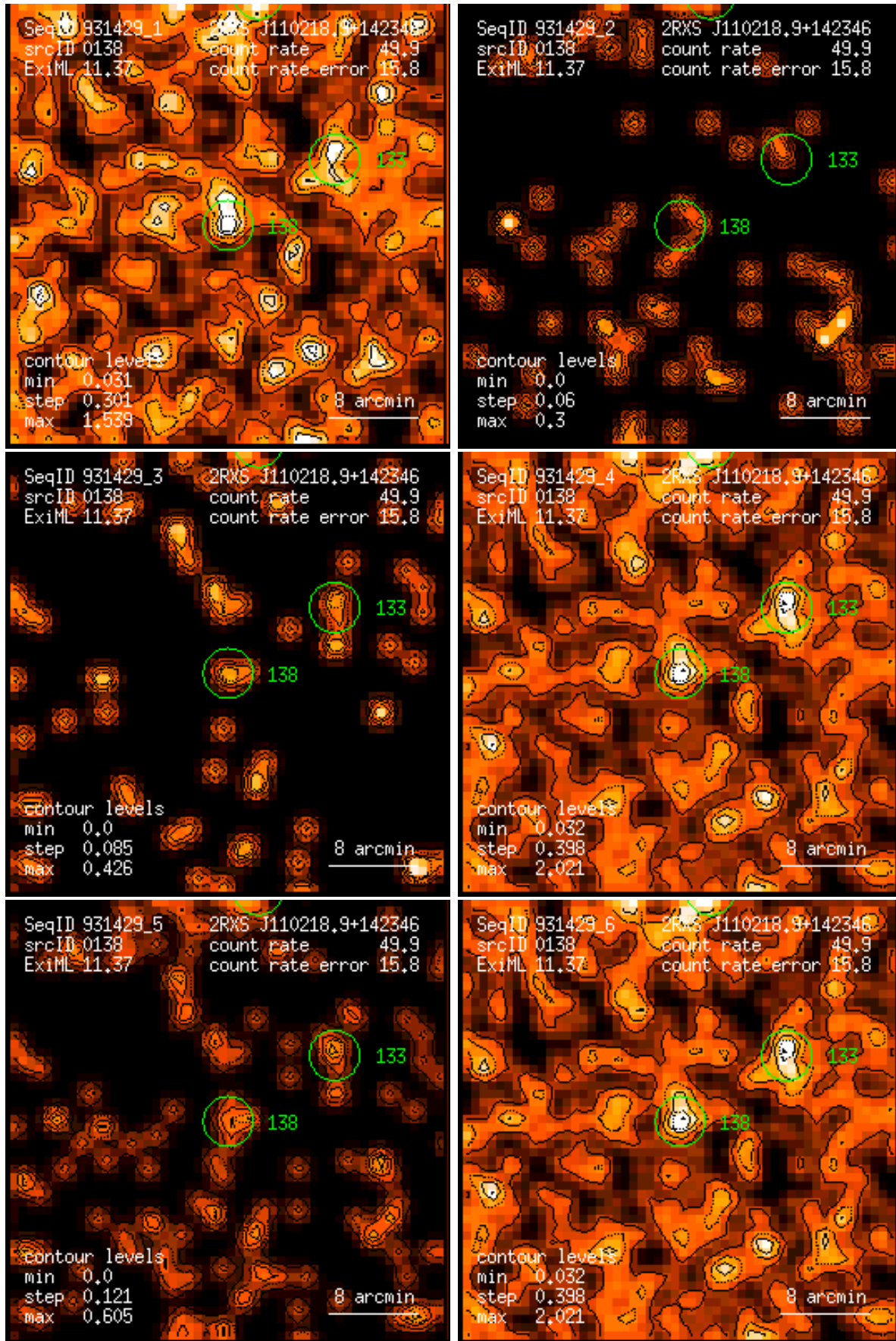
Figure 138: RASS 931429: detection 0138: band rate images, Gaussian filter: (1) PSPC channels 11 – 41, (2) 52 – 90, (3) 91 – 201, (4) 11 – 235, (5) 52 – 201, (6) 11 – 201. Broad band rates in counts/ks. Band rate contour levels in counts/ks/arcmin 2 .
