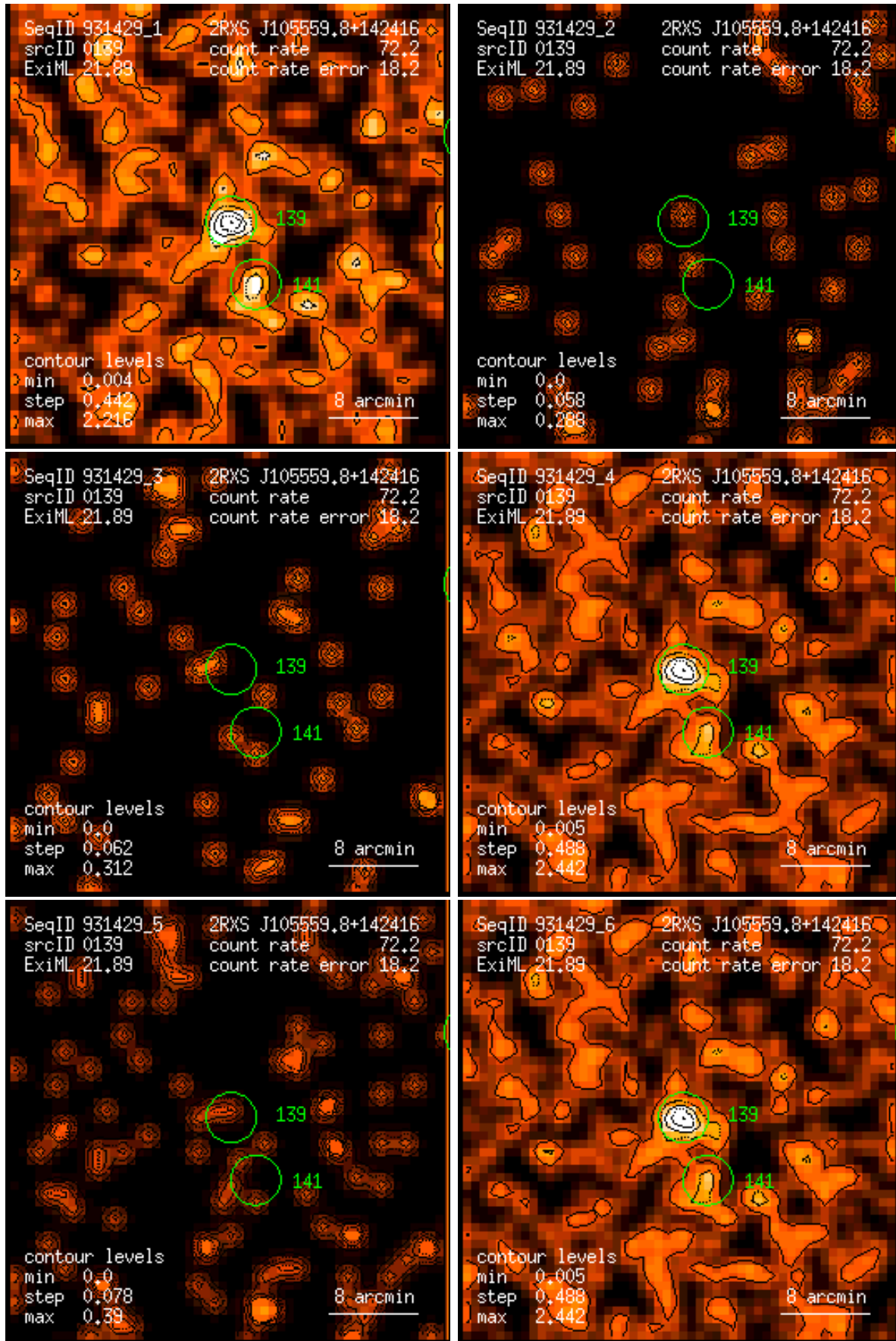
Figure 139: RASS 931429: detection 0139: band rate images, Gaussian filter: (1) PSPC channels 11 – 41, (2) 52 – 90, (3) 91 – 201, (4) 11 – 235, (5) 52 – 201, (6) 11 – 201. Broad band rates in counts/ks. Band rate contour levels in counts/ks/arcmin 2 .
