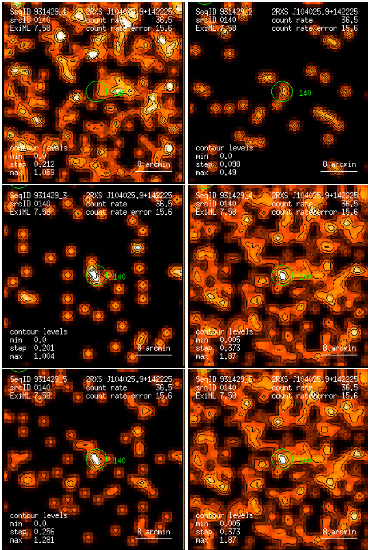
Figure 140: RASS 931429: detection 0140: band rate images, Gaussian filter: (1) PSPC channels 11 – 41, (2) 52 – 90, (3) 91 – 201, (4) 11 – 235, (5) 52 – 201, (6) 11 – 201. Broad band rates in counts/ks. Band rate contour levels in counts/ks/arcmin 2 .
