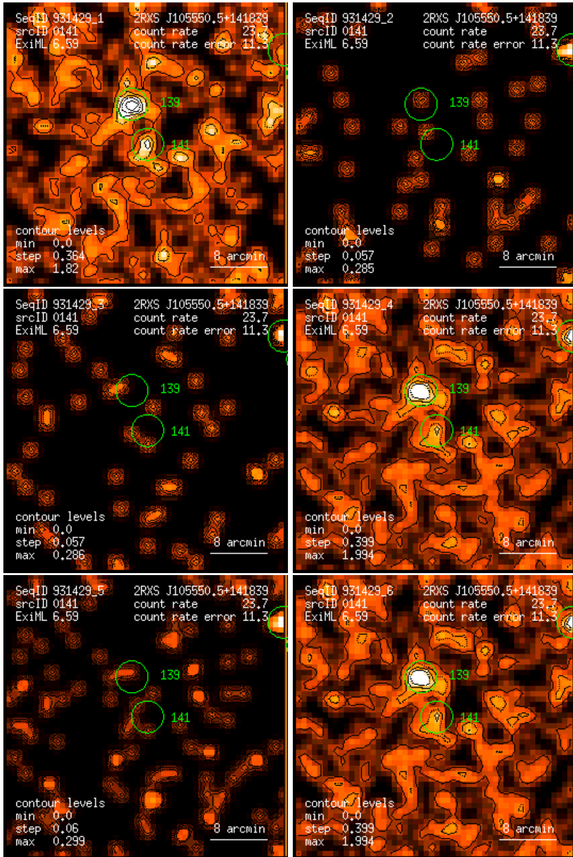
Figure 141: RASS 931429: detection 0141: band rate images, Gaussian filter: (1) PSPC channels 11 – 41, (2) 52 – 90, (3) 91 – 201, (4) 11 – 235, (5) 52 – 201, (6) 11 – 201. Broad band rates in counts/ks. Band rate contour levels in counts/ks/arcmin 2 .
